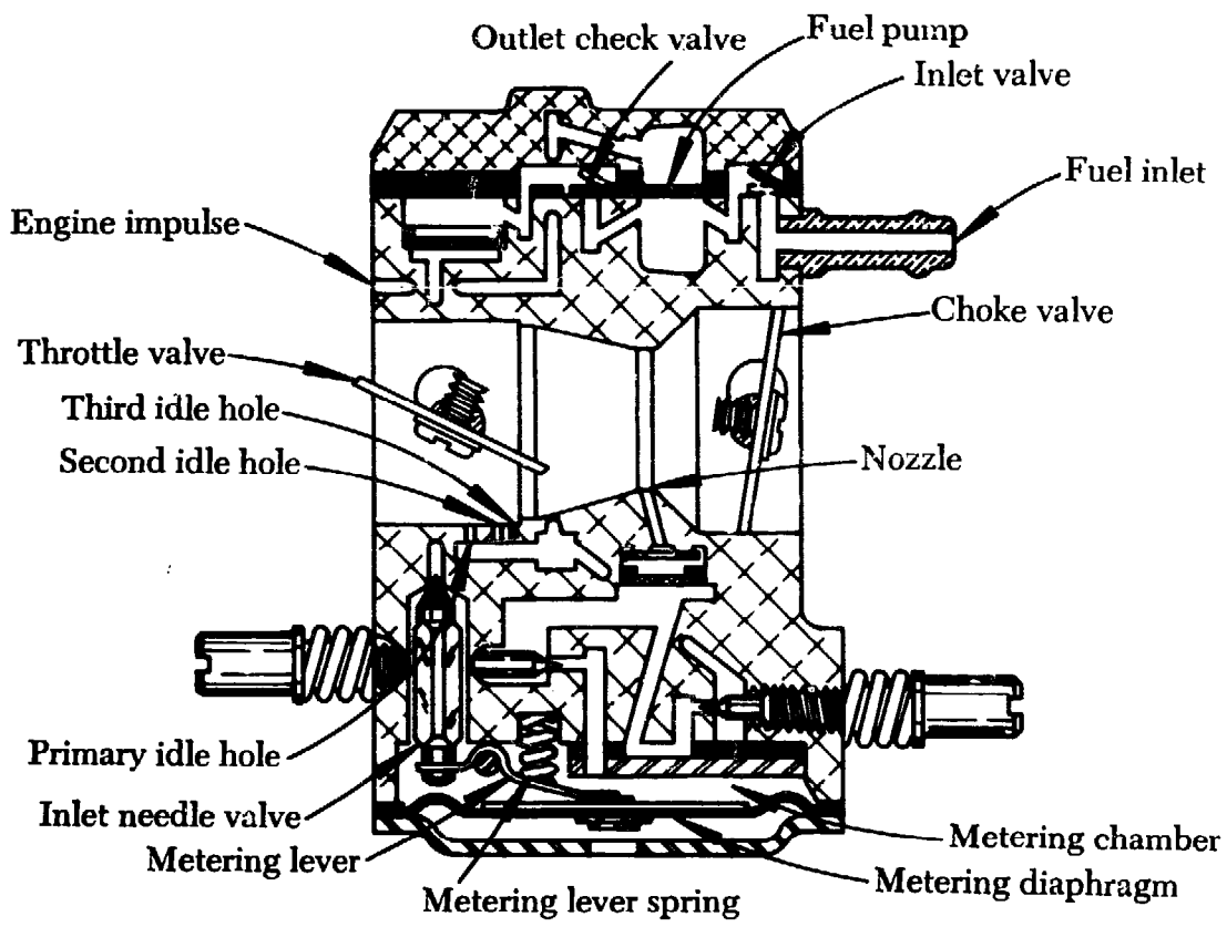
Starting phase of typical Walbro chain saw carburetor Figure 9.7
