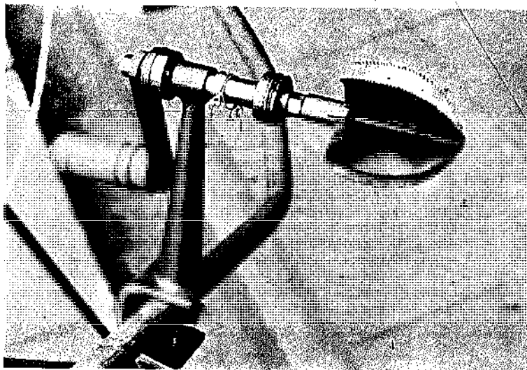
"Lucky Meri Super Scraper" coconut scraper, using front axle and bearing of bicycle wheel from New Britain Engineering, P.O. Box 163 Rabaul. Price K7.50 plus shipping.
