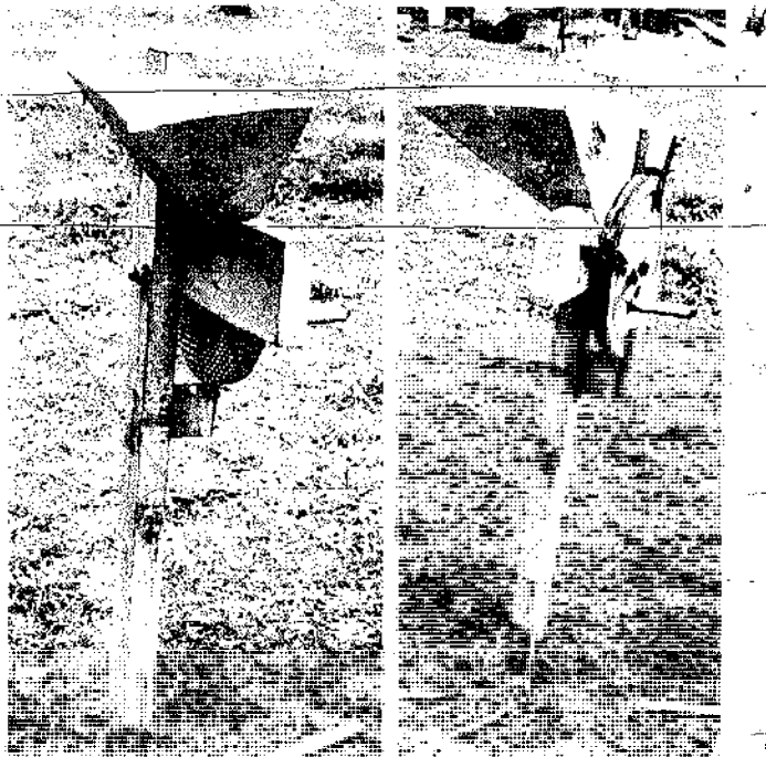
Home made coffee pulper made of wood, tin, and a few odds and ends. More information from Village Development Office, Box 6937, Boroko.
