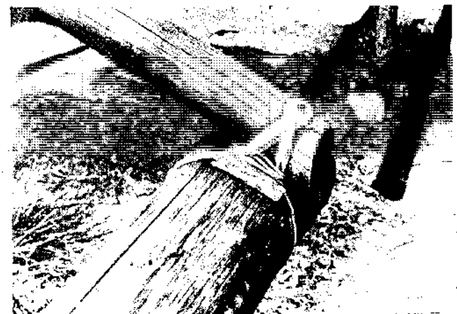
11. The bamboo runners are attached to the arms with heavy nylon fishing line. Note brass nail in top of bamboo arm and piece of old slipper between two bamboos. A thick-walled durable kind of bamboo is used.
