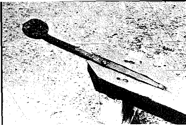
Very common type of coconut scraper found in the Philippines. Made from 13 mm (1/2") round bar.
