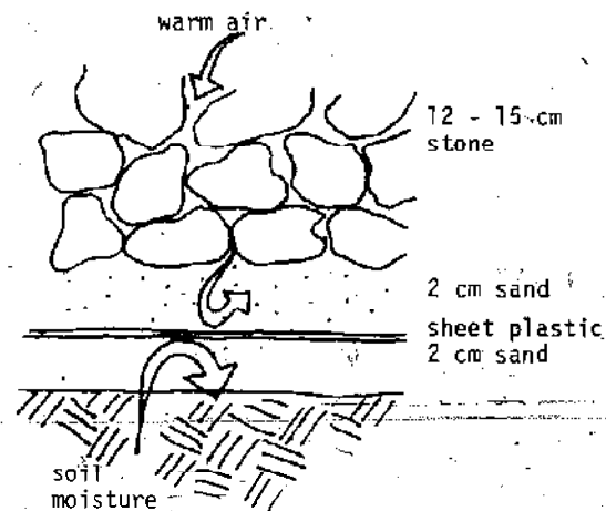
The effect of sheet plastic in the insulated floor.
