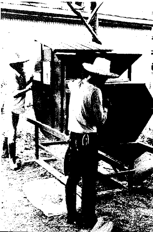
Tradition Central Luzon Philippines model winnowing machine, plans available from International Rice Research Institute, Box 933, Manila, Philippines.
