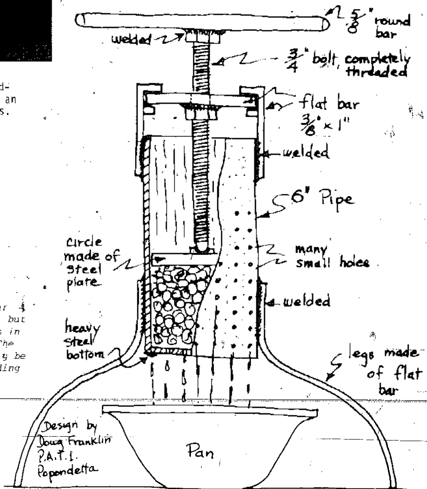
Design by Doug Franklin P.A.T.I. Ponondetta Pan SIMPLE OIL PRESS (cutaway view)
