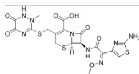
Structural formula of ceftriaxone, one of the third-generation cephalosporin antibiotics recommended for the initial treatment of bacterial meningitis.
