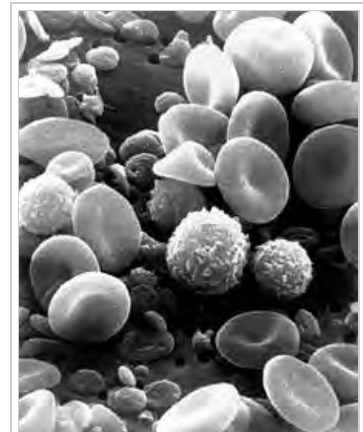
A scanning electron microscope image of normal circulating human blood. One can see red blood cells, several knobby white blood cells including lymphocytes, a monocyte, a neutrophil, and many small disc-shaped platelets.
