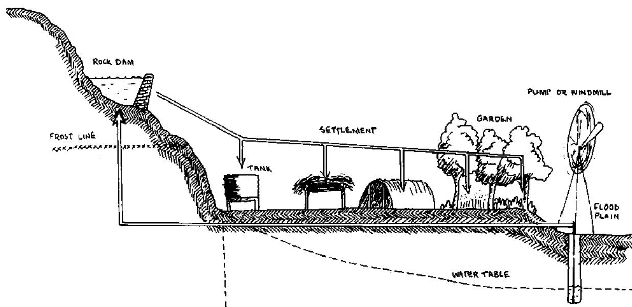
FIG. 5.2: IDEAL RELATIONSHIPS — WATER, SETTLEMENT, GARDENS FOR ARID LANDS
