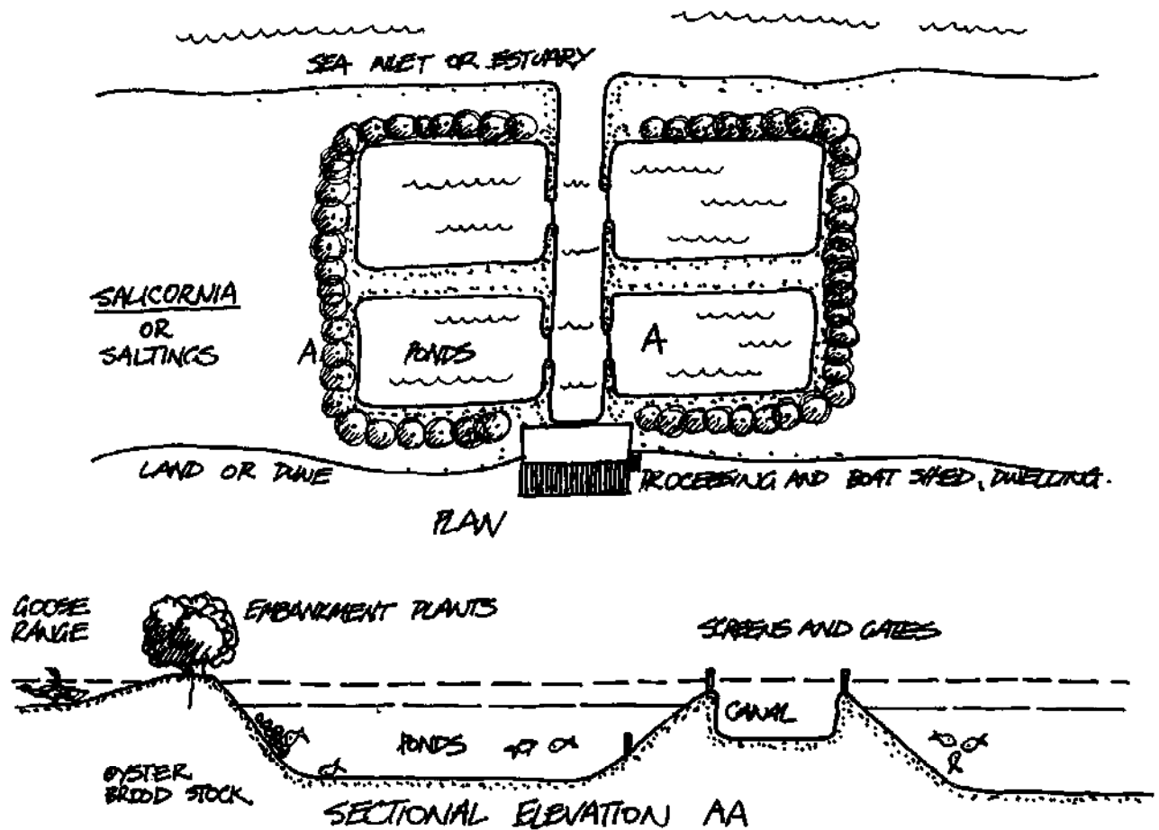
FIG. 7-24: PLAN AND SECTION OF TIDAL POOLS.
