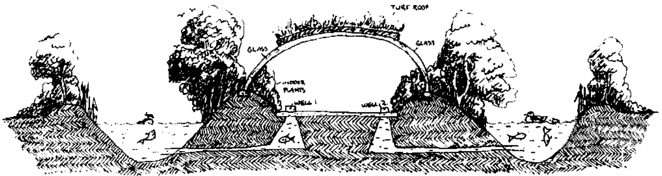
FIG. 6.6 SECTION OF EARTH HOUSE - LIGHT INDOOR DIVISIONS CAN BE MADE. END WALLS OF GLASS TO NORTH, SOLID TO SOUTH.
