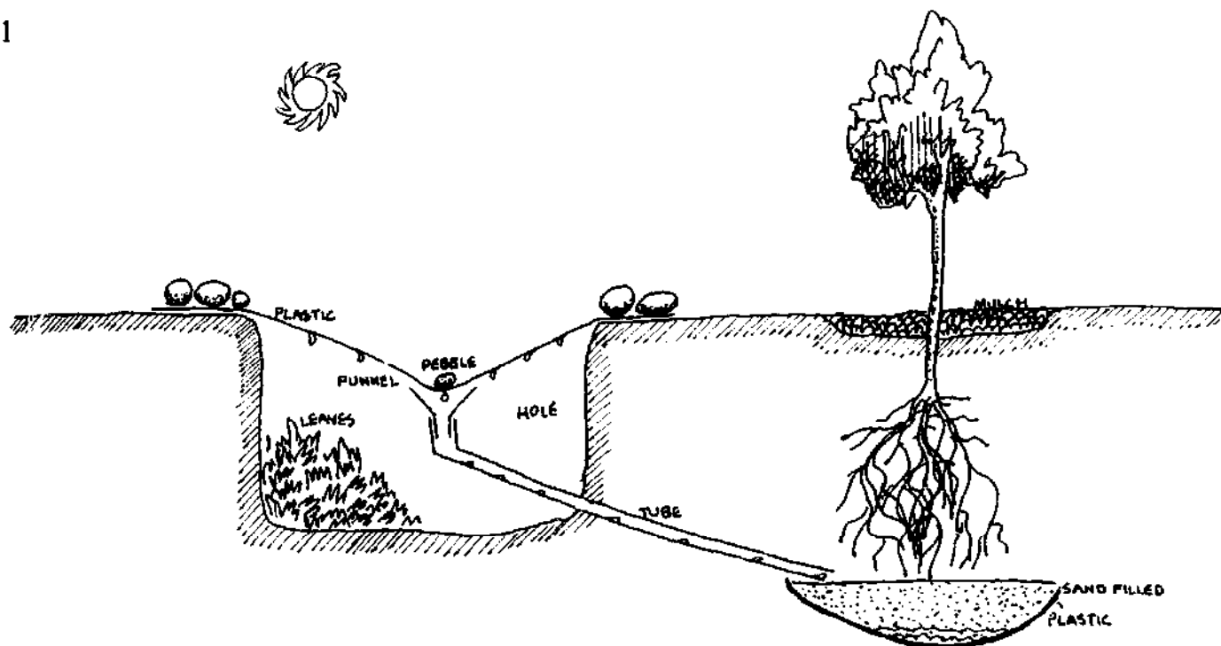
FIG.5:20: PLASTIC STILL USES LEAVES OR SOIL TO DISTILL WATER FOR PLANT RESEVDIR..
