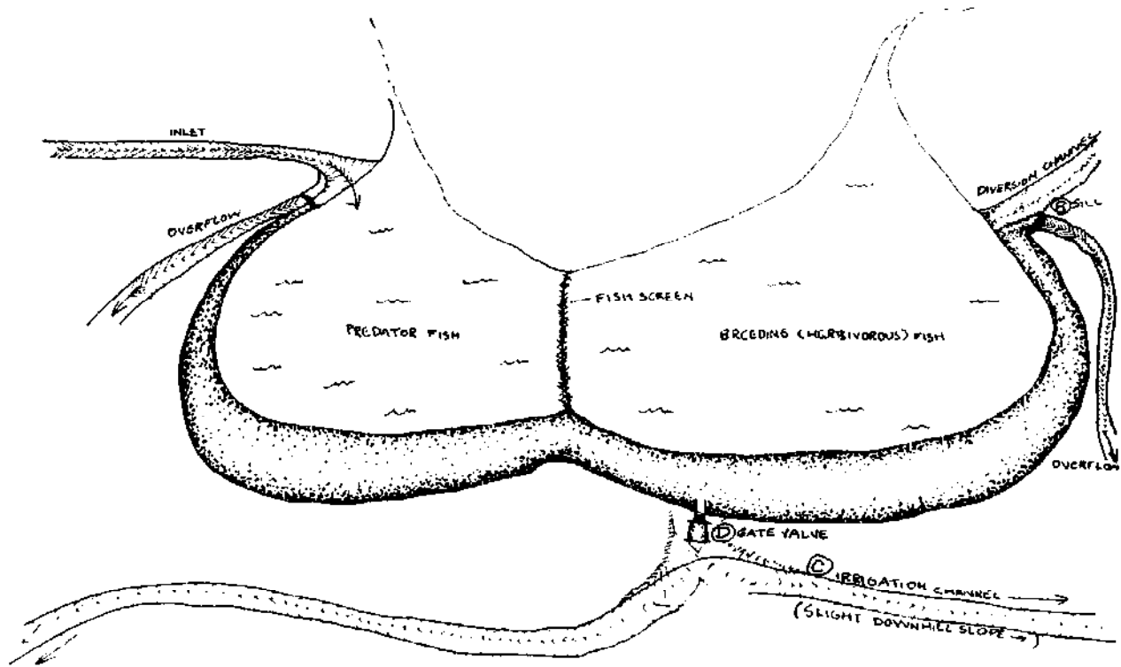
FIG. 7.12: "DOUBLE" DAM IN DEPRESSION CONNECTED VIA FISH SCREEN. PREDATORS (TROUT) KEEP HERBIVORES (PERCH) CULLED VIA FISH SCREEN (YANDOTT, VICTORIA)
