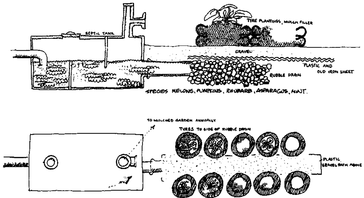
FIG. 6:20: DISPOSAL OF SEPTIC TANK EFFLUENT OR SOLLAGE VIA TYRE-PLANTED ROWS.
