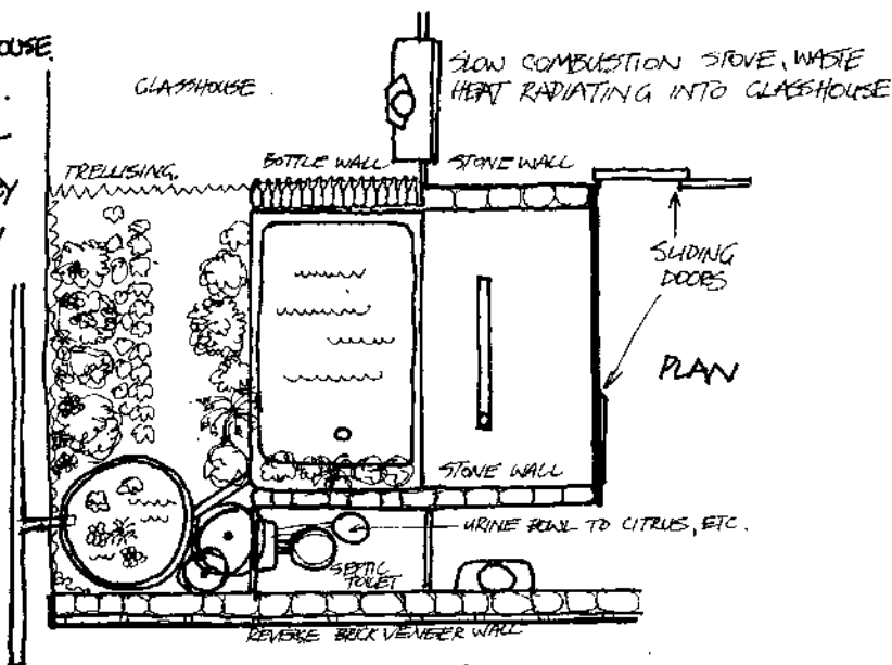
FIG. 6-13: BATHROOM GLASSHOUSE. SHOWER OVER TUBBLE BED KEEPS PLANTS MOIST. CAN BE ATTACHED TO EXISTING BATHROOM AS 'HOT' OR 'COLD' GLASSHOUSE.
