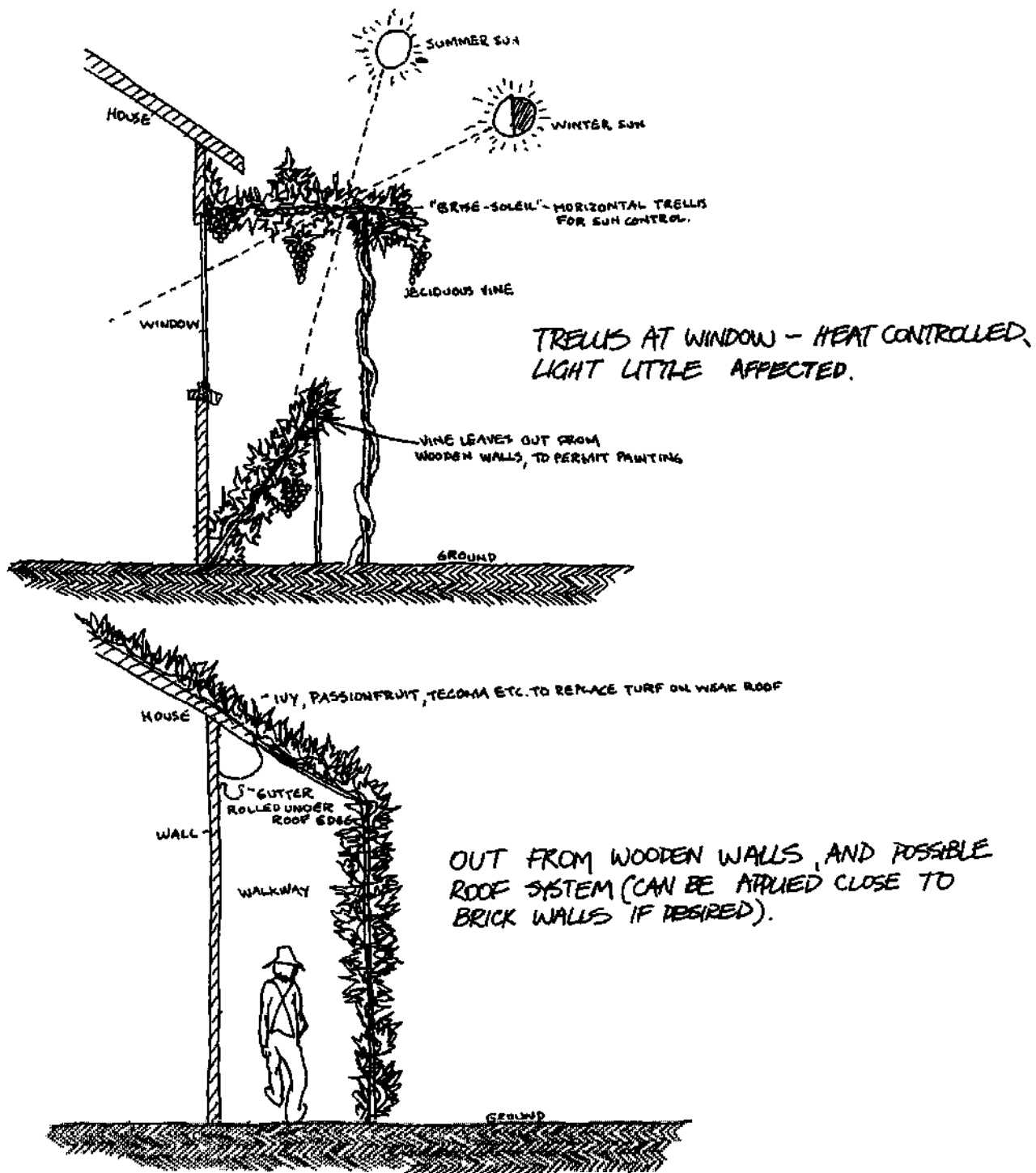
WALL TRELLIS FOR INSULATION FROM WIND AND HEAT. FIG. 6.15
