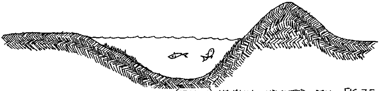
TYPICAL EARTH BANKS OF FLATLANDS (SECTION). USUALLY UNPLANTED, OPEN TO WIND AND EVAPORATION. OFTEN WASTE SUBSOIL IS HEAPED ON THE SUN SIDE AND STOCK CAN APPROACH FROM ANY QUARTER MUDDYING WATER. FIG. 7.5
