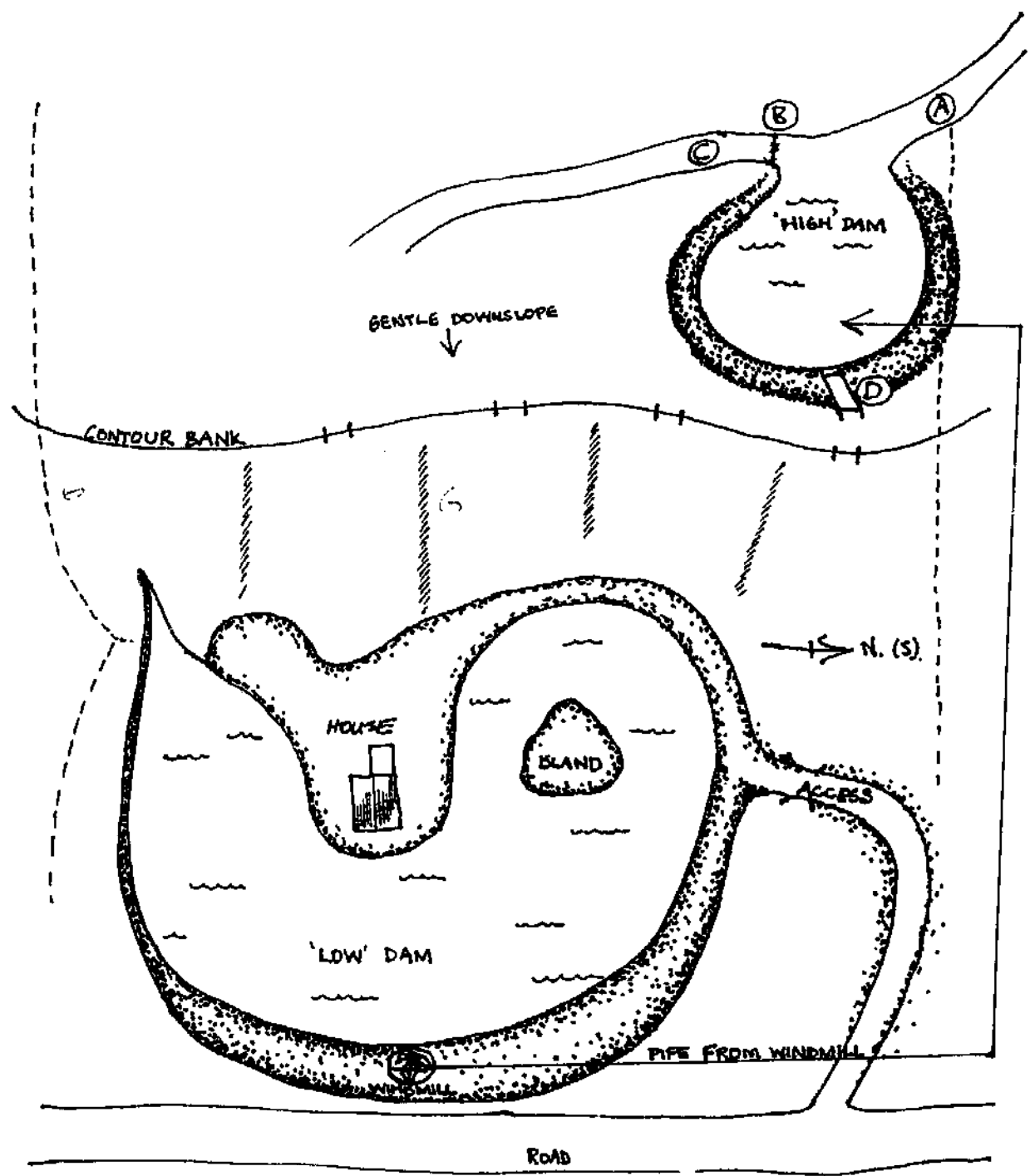
LAYOUT OF 5 ACRES AT DICGER'S REST, VICTORIA. HOUSE PROTECTED FROM FIRE, WHOLE AREA WATER CONTROLLED. DESIGNED BY YEDMANS, GALL AND MOLLISON. (SEE DETAIL FIG. 7.14.)
