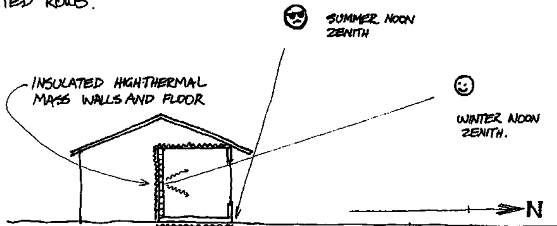
FIG 6:21: SUN/WINDOW/EAVE RELATIONSHIP.
