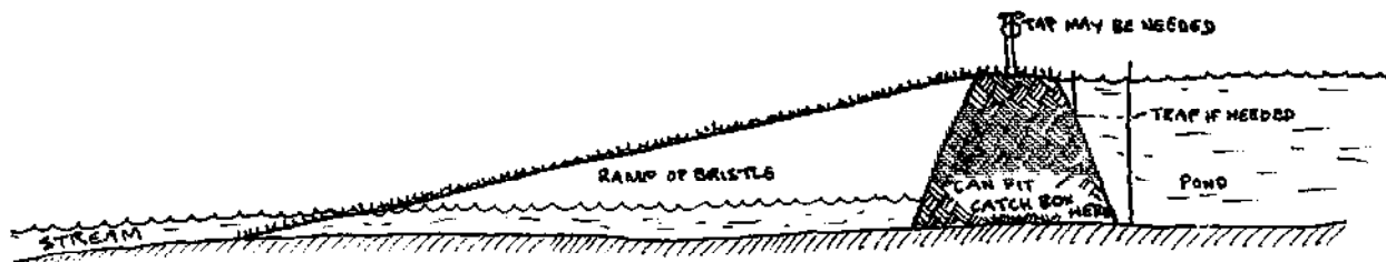
A SLOPE OF NYLON BRUSH BRISTLE, OR TURF, OR ROUGH STONE FOR WRIGGLING AND CREEPING SPECIES SUCH AS EELERS, YABBIES, SHRIMPS, ETC (AFTER MODEL AT LIMERICK, IRELAND).
