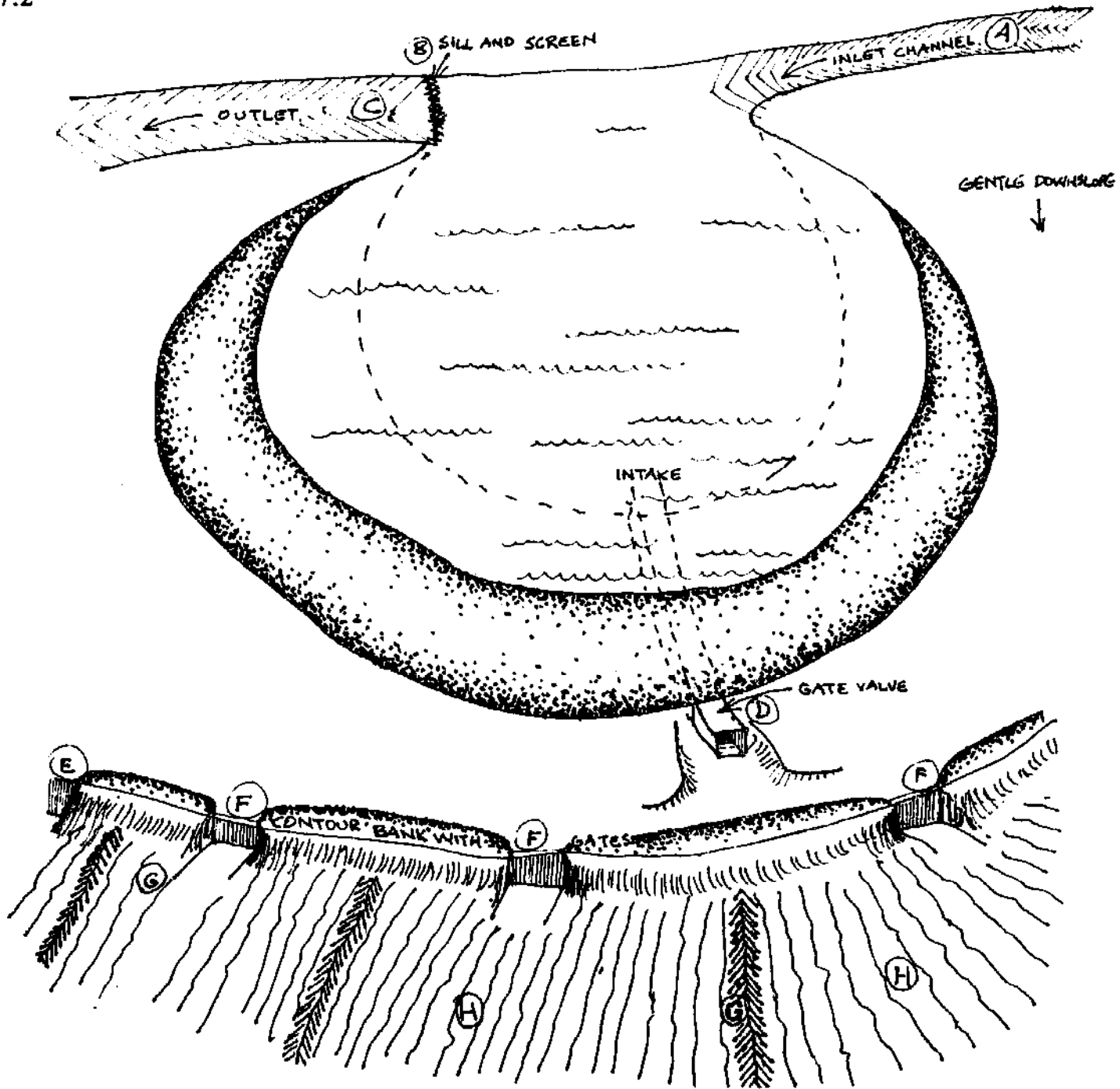
FIG. 7.14: HIGH HOLDING DAM GATHERS WATER AT (A) FROM A 1:150 LEAD IN (DIVERSION) DRAW ACROSS SLOPE. IN FLOOD, THIS LEAD IN WATER SPILLS ACROSS SILL (B) TO OUTLET CHANNEL (C) OR CAN BE RELEASED THROUGH GATE VALVE (D) AT ANY TIME. CONTOUR BANK (E) HOLDS RELEASED WATER FOR CONTROLLED LIBERATION INTO FIELDS (H) VIA GATES (F). WATER IS THEN CONTROLLED BY VERY LOW STEERING BANKS (G), AND SOAKS INTO CHISEL PLOUGHED FIELDS. DIRECTION OF CHISELLING INDICATED BY WIDE-SPACED LINES. (AFTER DAM AT DIGGER'S REST DESIGNED BY KEN YEOMANS).
