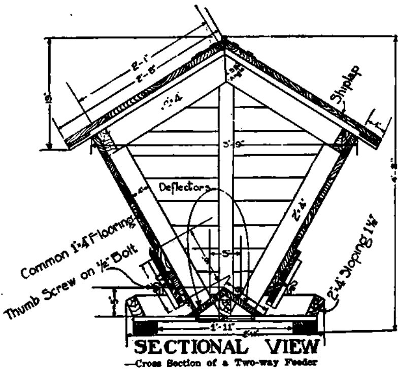
FIGS. 191-192.—A two-way feeder used by the Missouri Agricultural College. Bulletin 144.
