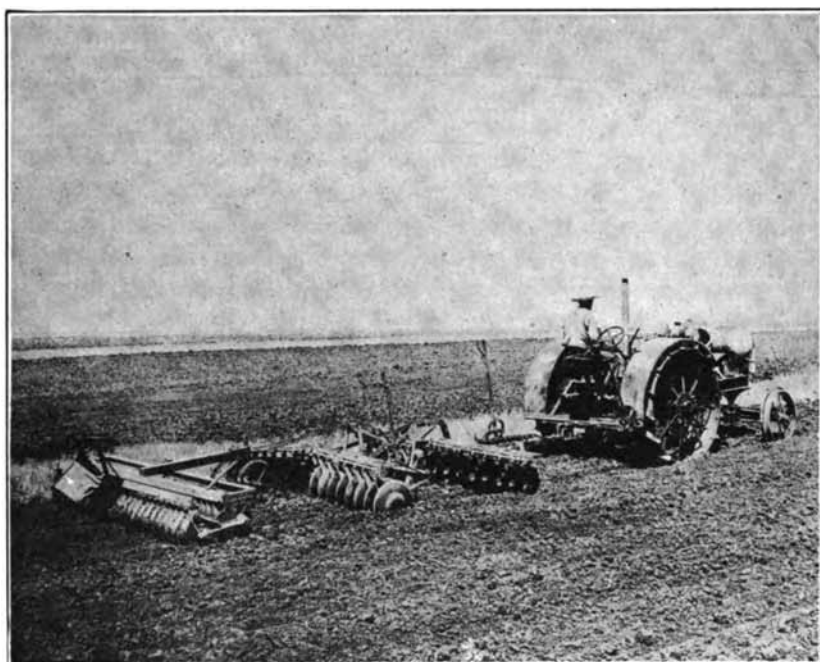
FIG. 4.—Cutting, pulverizing and compacting the seedbed at one operation.— By permission of Dunham Co., Berca, Ohio.
