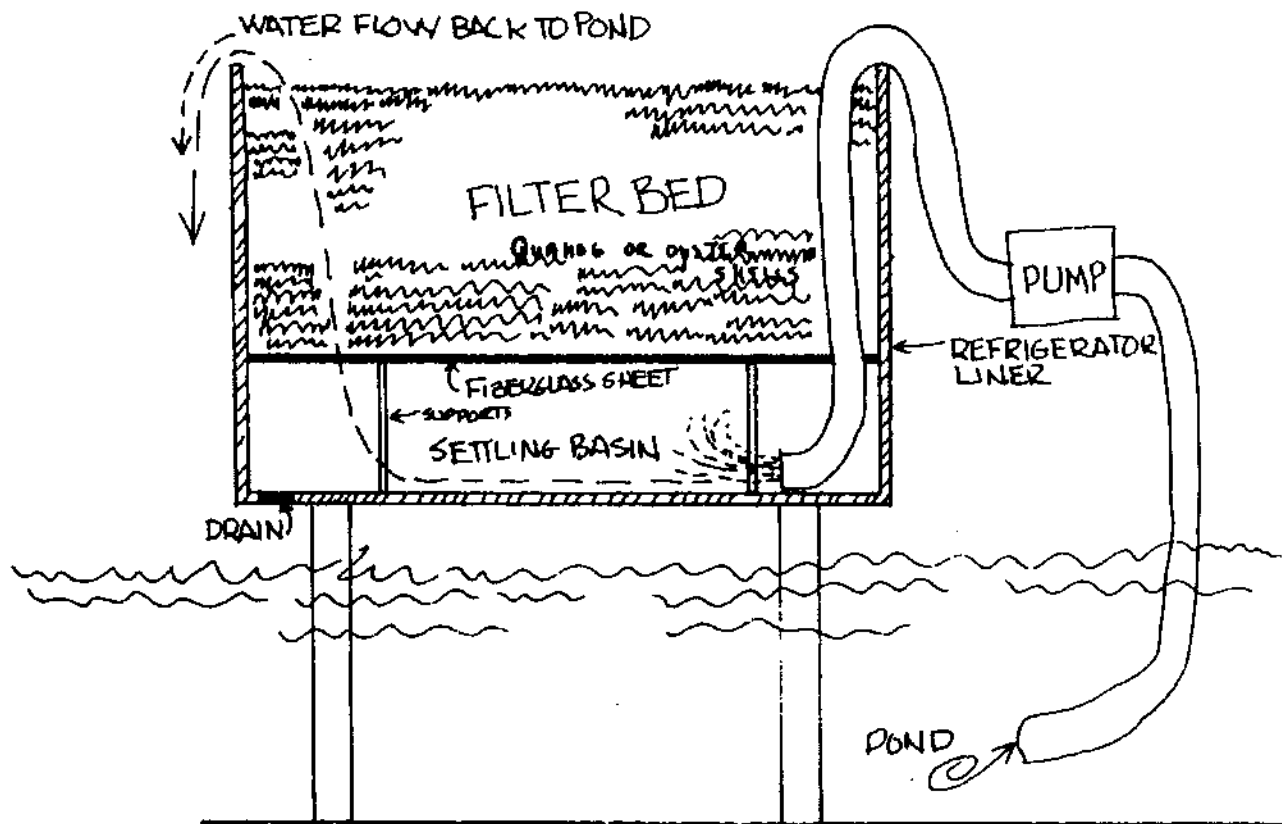
Fig. 5 — Filter
