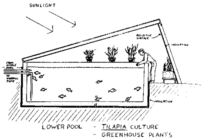
Fig. 13 Greenhouse - Fish Culture Structure
