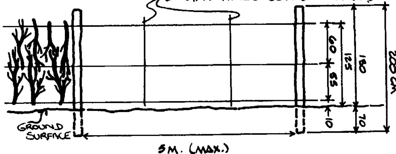
STANDARD 3 STRAND FENCE (NOTE: MINIMUM IMPORTED MATERIALS)
