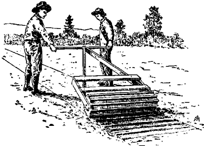
FIG. 32. Concrete marker-roller.
