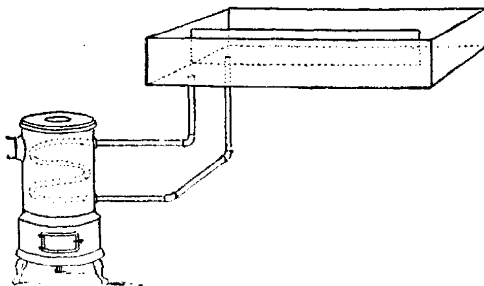
FIG. 83. Barnard's propagating-tank.
