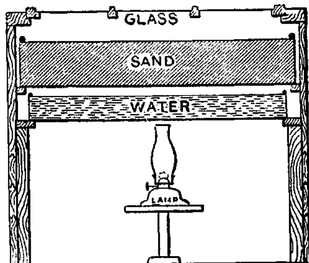
FIG. 82. Simple propagating-oven.
