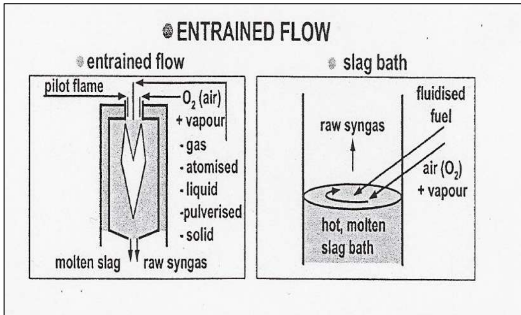
Fig. 3.3: Entrained gasifier
