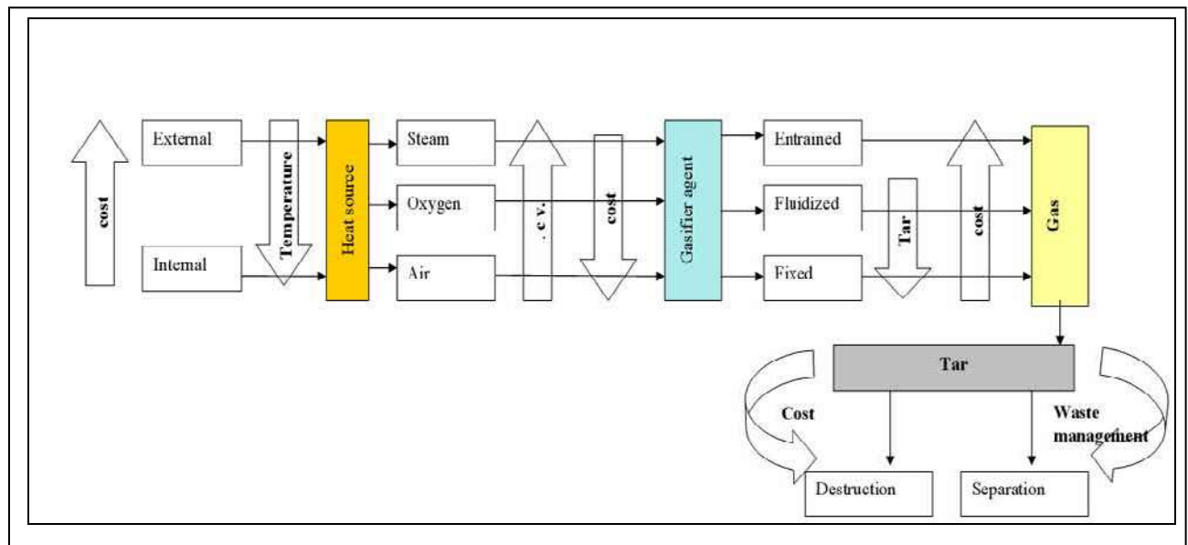
Fig. 3.2: Gasification process overview
