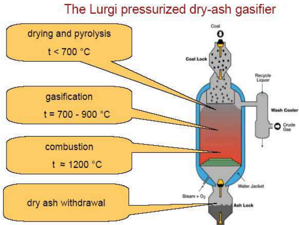
Figure (1-5): The Lurgi Dry Ash Gasifier.
