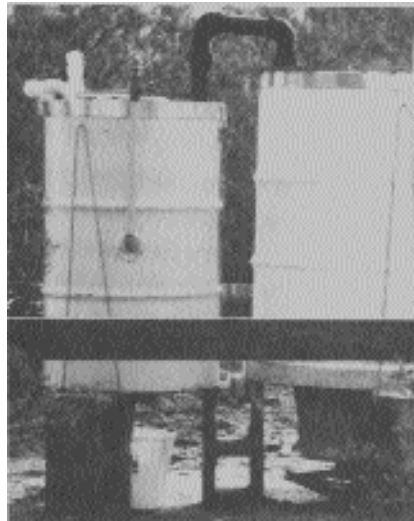
Converted oil drums make up the upright gas producer, right, and gas scrubber.
