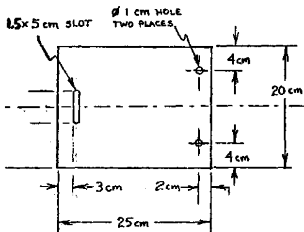
HASP PLATE (Make from barrel bottom)
