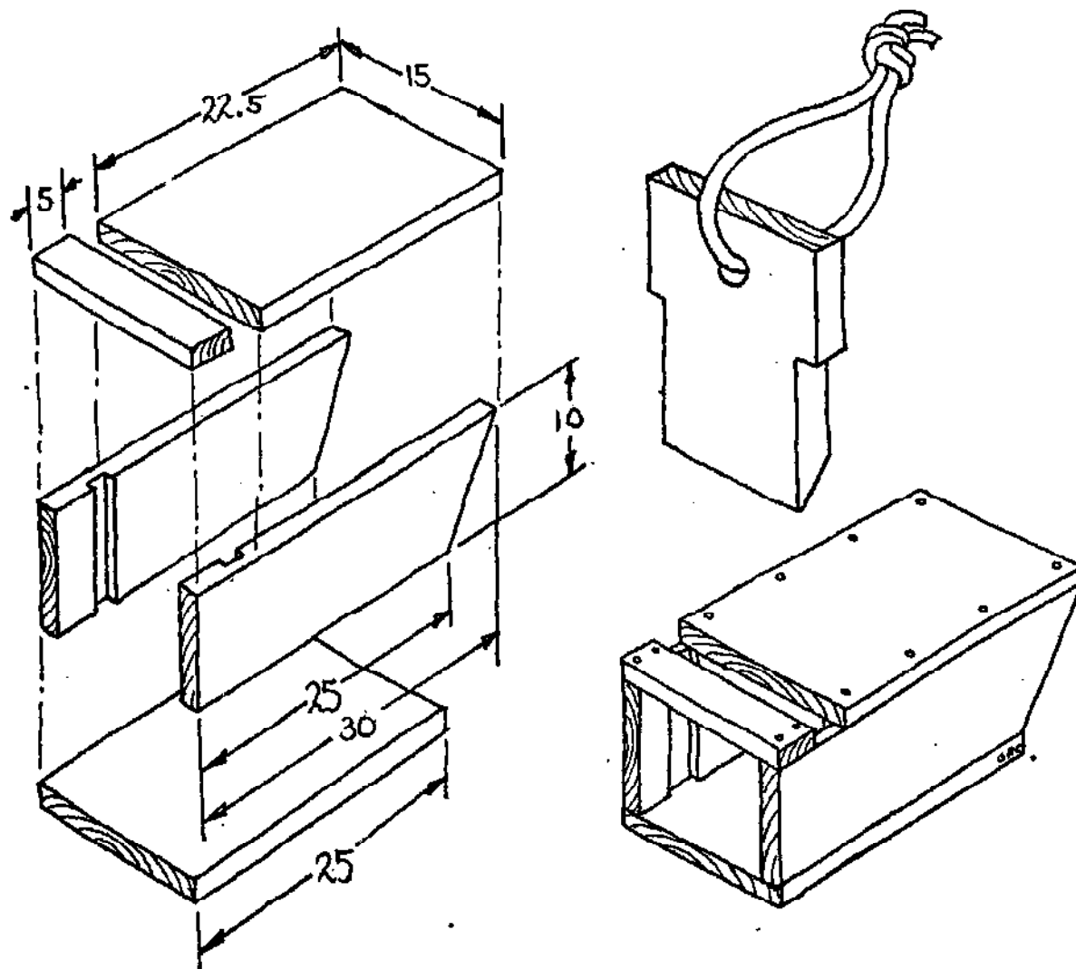
GRAIN CHUTE
