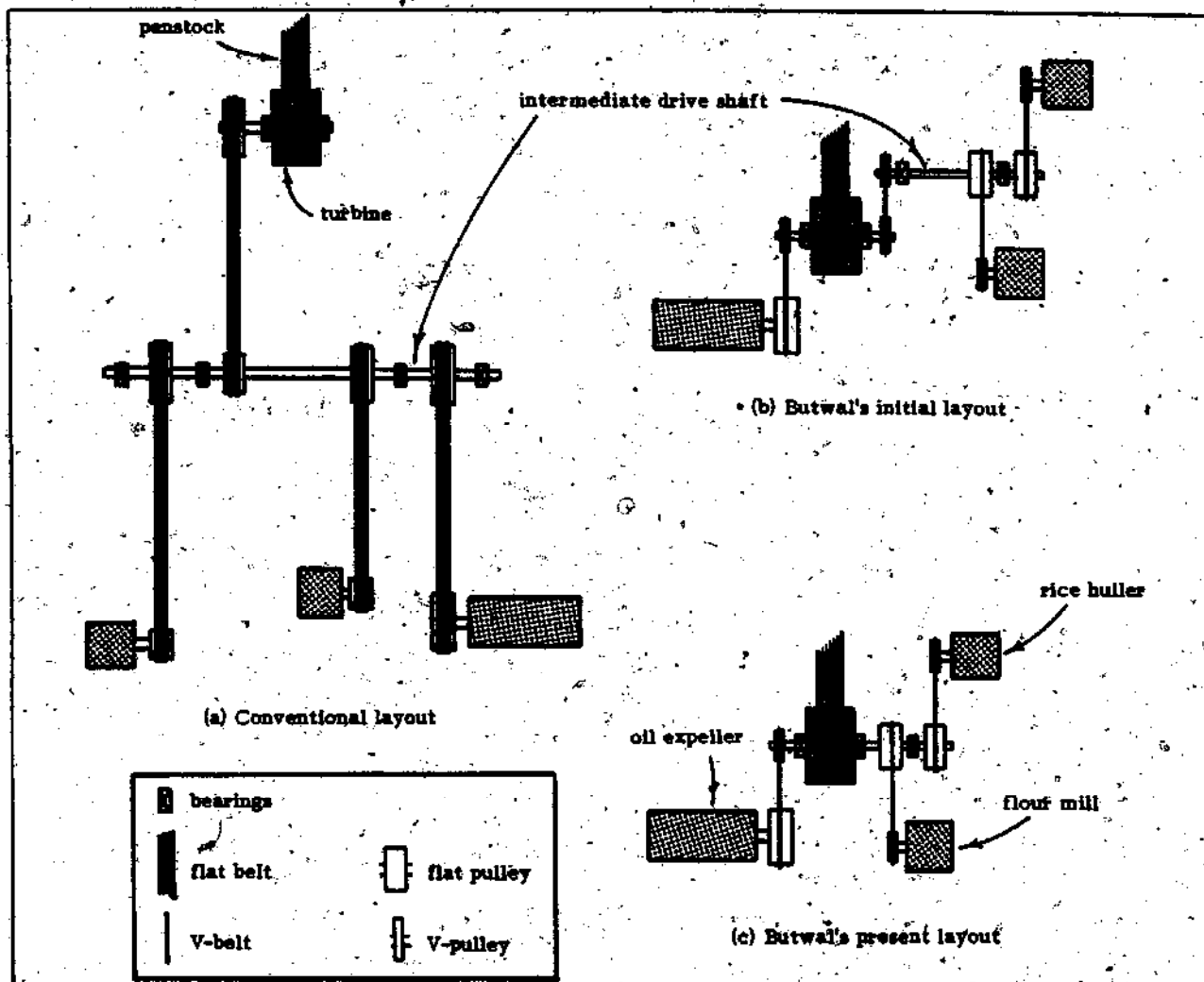
Fig. 18. These drawings illustrate the evolution of the standard equipment layout in a mill. Note that the floor area is reduced as are the number of bearings and the overall complexity.
