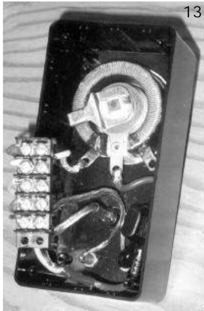
Fig. 13: Draw a wiring diagram and check it against the schematic before you start construction.
