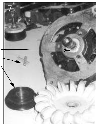
Front bearing Brush springs Impeller plate
