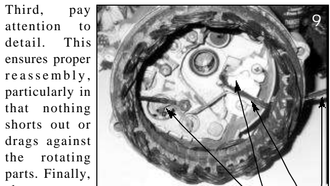
Stator lead Brush holder Grocery tie for brushes
