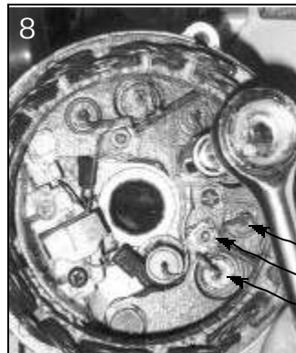
8. The nut is removed from a stator terminal to free two diode leads.
