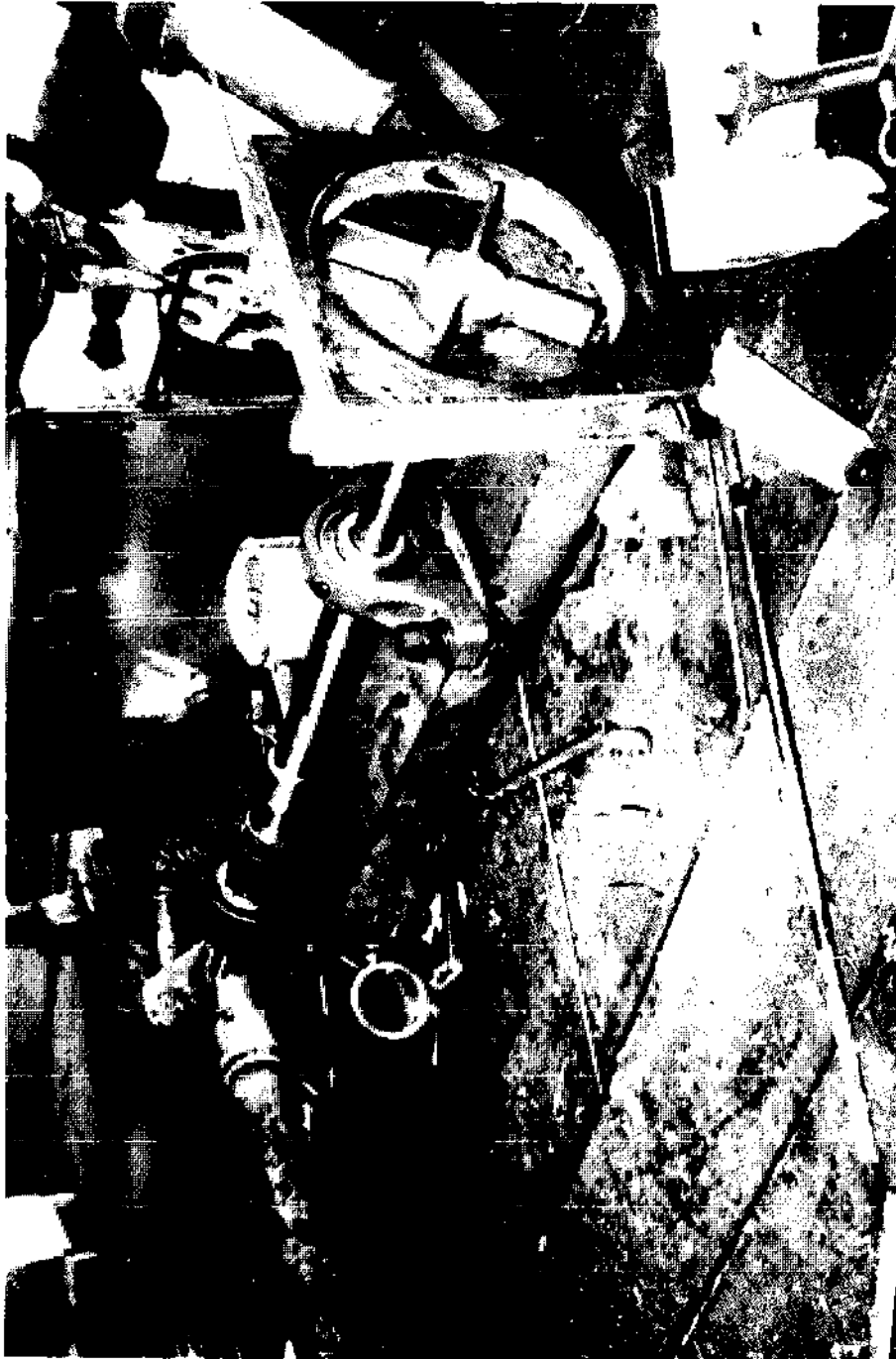
FIGURE 2.15: Locally Fabricated Pump for 'Low Cost' Turbine.
