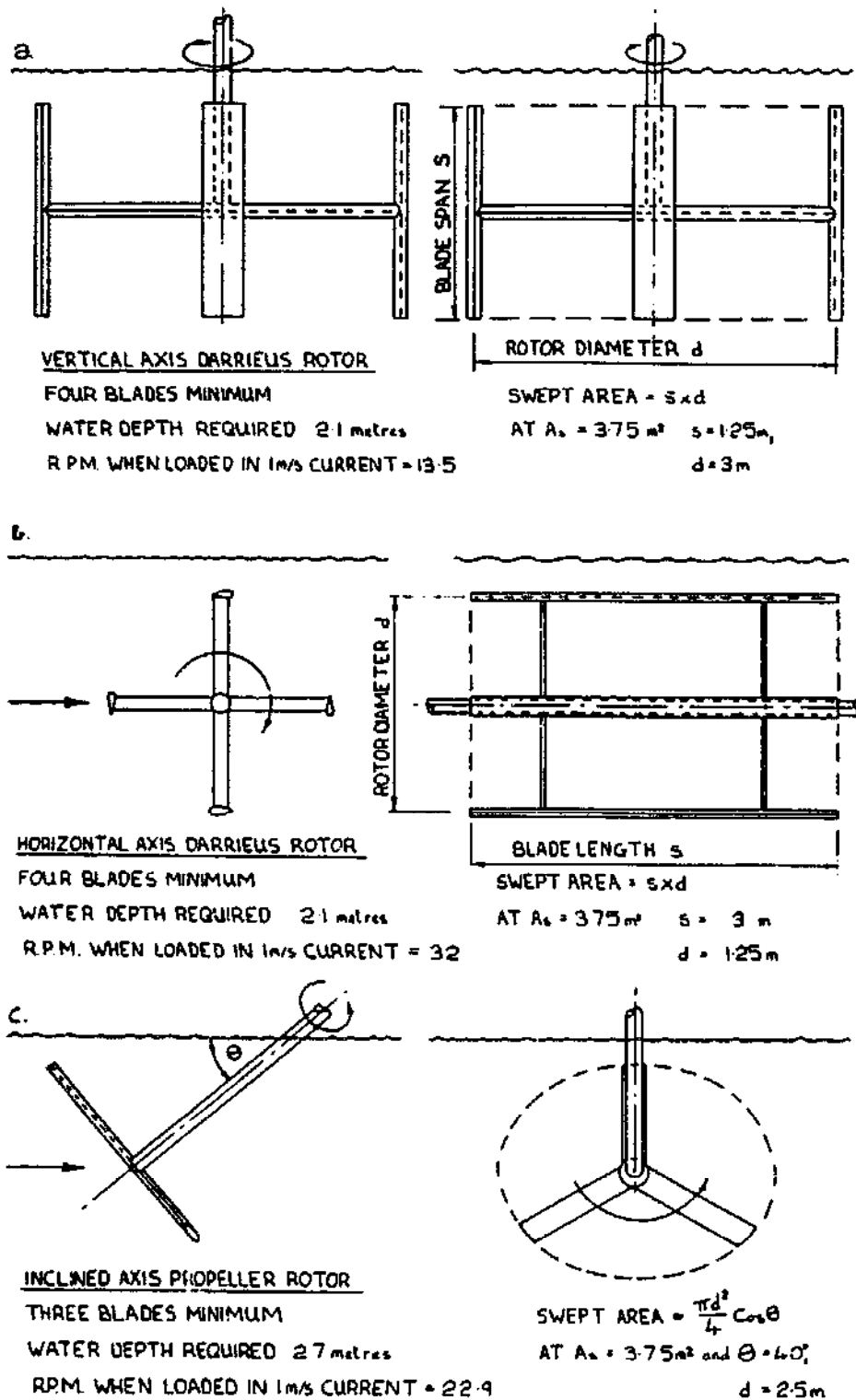
FIGURE 2.7: Sketches of Alternative Turbine Rotors.
