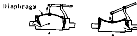
Fig.51 Cross-section of a diaphragm pump
