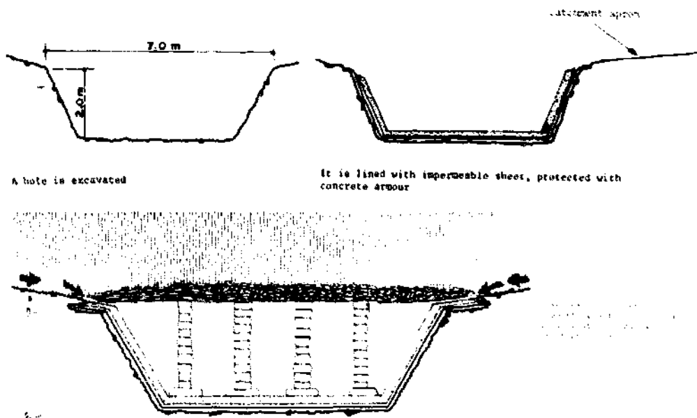
Fig.29 Catchment tank construction
