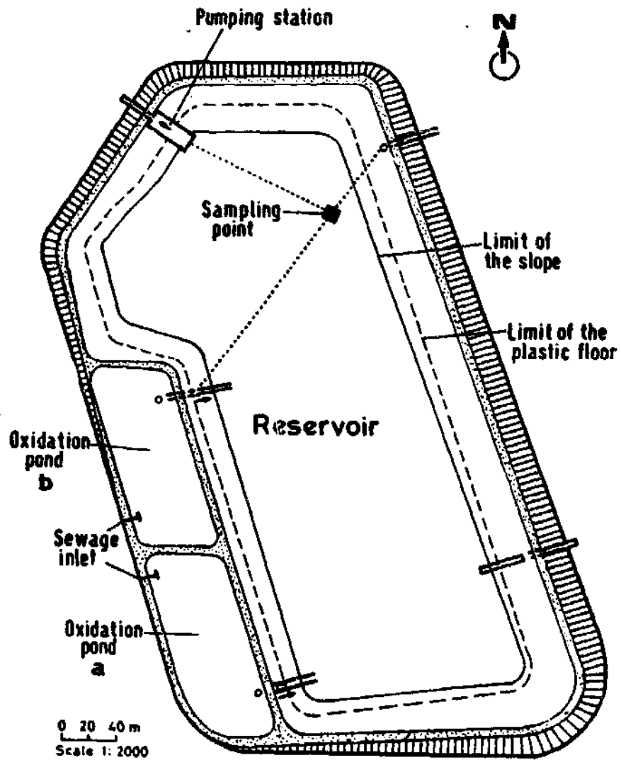
Fig. 5-2. Schematic layout of Maan Wastewater Reservoir, Israel. Source: Adapted from Dor and Berend (1982).
