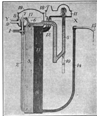
FIG. 207.—Diagrammatic Sketch of Forbes Water Sterilizer—A. my Type.
