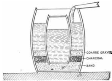
FIG. 214. — Improvised Filter.
