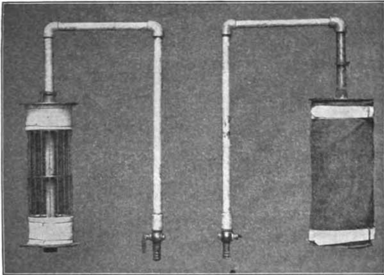
FIG. 210.—Darnall Filter. Showing two siphons, one without filter cloth.
