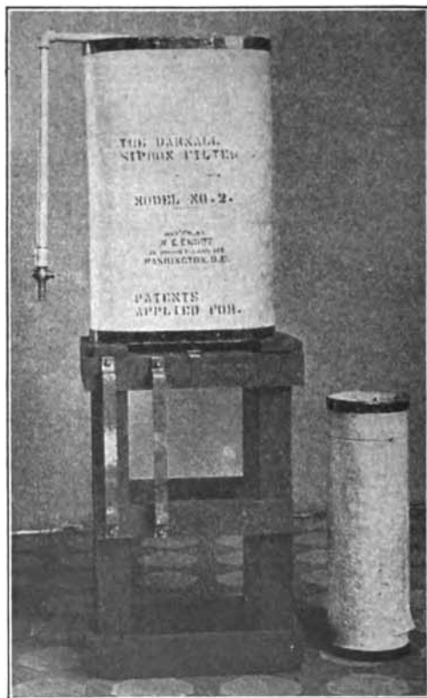
FIG. 209.—Darnall Filter. Set up ready for use.
