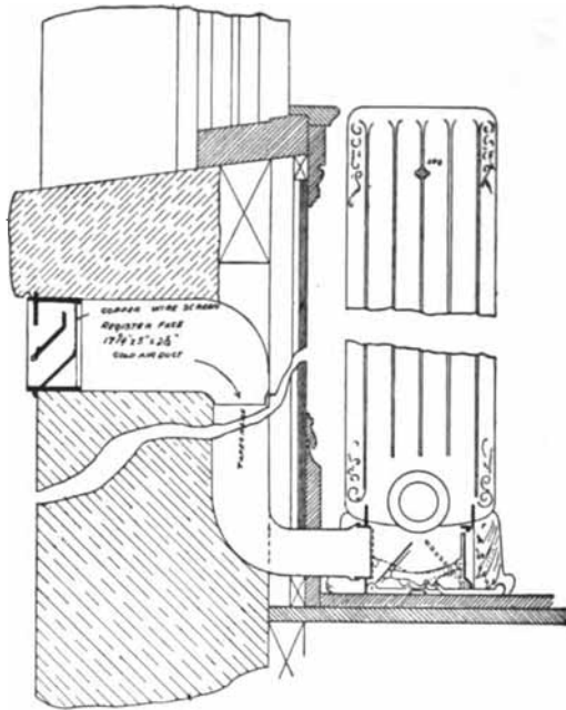
FIG 218.— Heating by Direct-Indirect Method.
