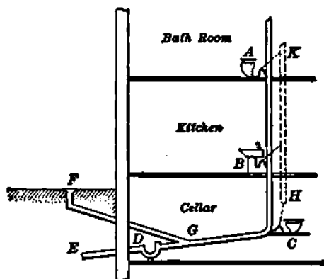
FIG. 219.—House Drainage. A, B, C , Plumbing fixtures; D , disconnecting trap; E , branch sewer; F , ventilation opening; G , house drain; K, H , vent pipes connected by dotted lines with each trap.
