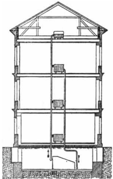
FIG. 216.—Heating by Hot Water. Low pressure.
