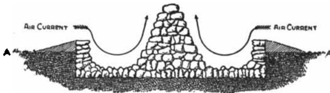
FIG. 229.—Crematory—Vertical Section. A A, Ground level.
