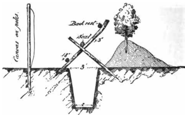
FIG. 223.—Field Sink.
