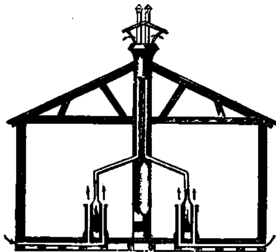
FIG. 215.—Heating and Ventilation by Jacketed Stove.
