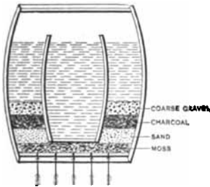
FIG. 213. — Improvised Filter.
