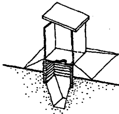
Fit latrine on mound with sealed brick to 2 feet below ground level. Useful in wet ground.
