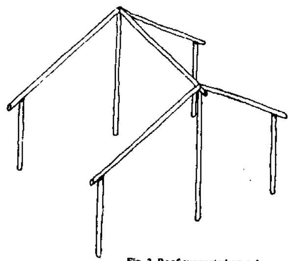
Fig. 3 Roof supported on columns
