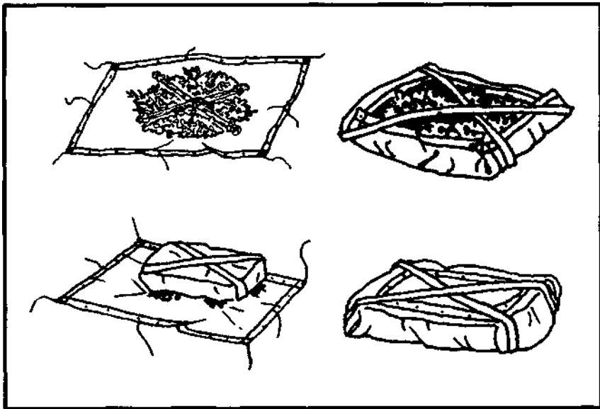
Figure 17-4. Brush raft.
