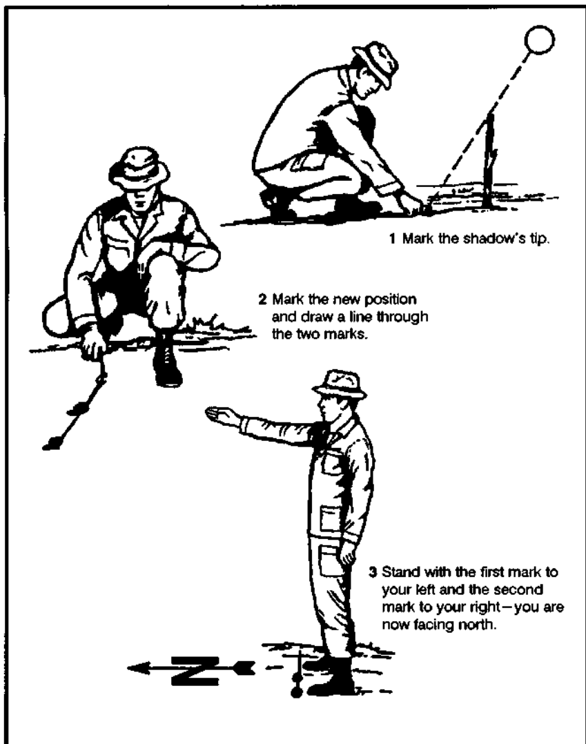
Figure 18-1. Shadow-tip method.
