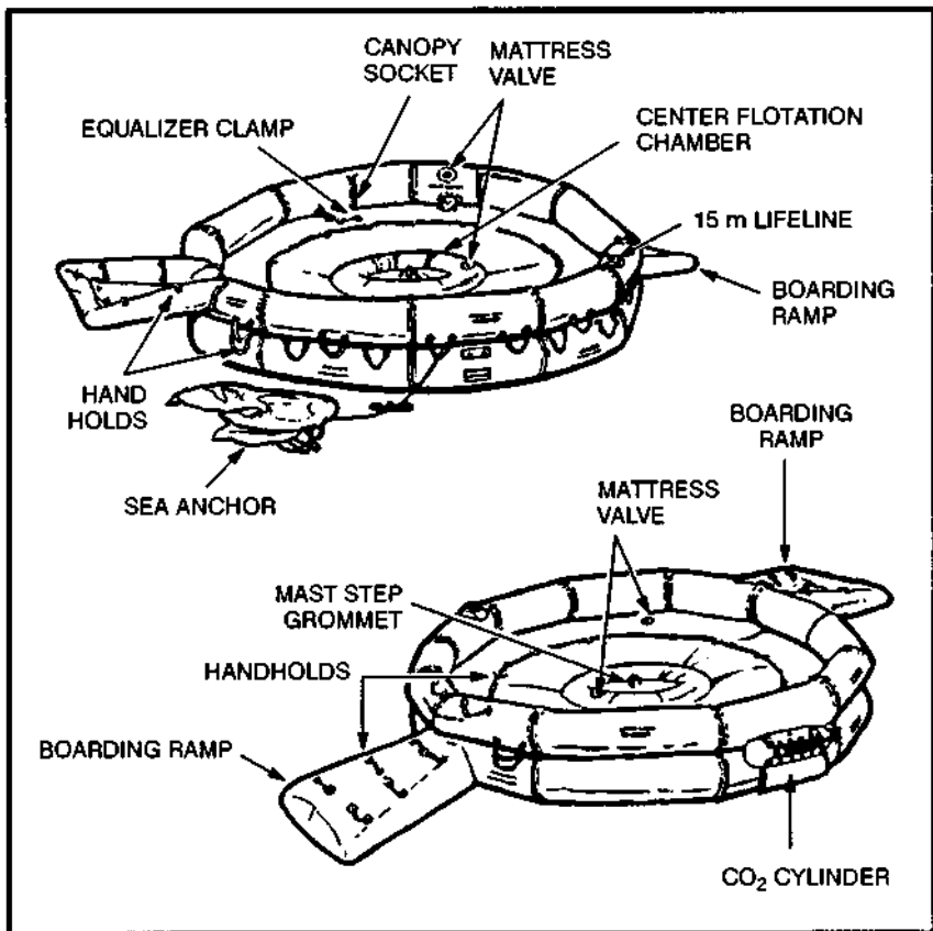
Figure 16-15. Twenty-man raft.
