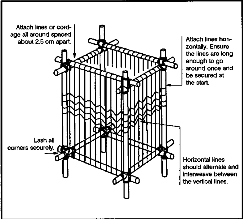
Figure 12-10. Square pack.
