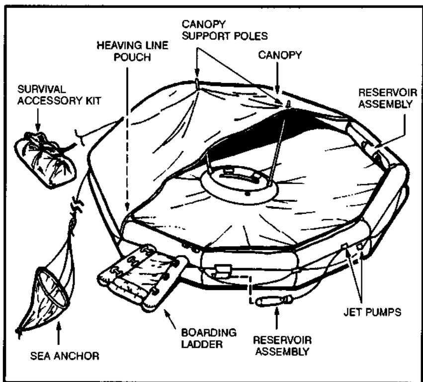
Figure 16-16. Twenty-five-man raft.
