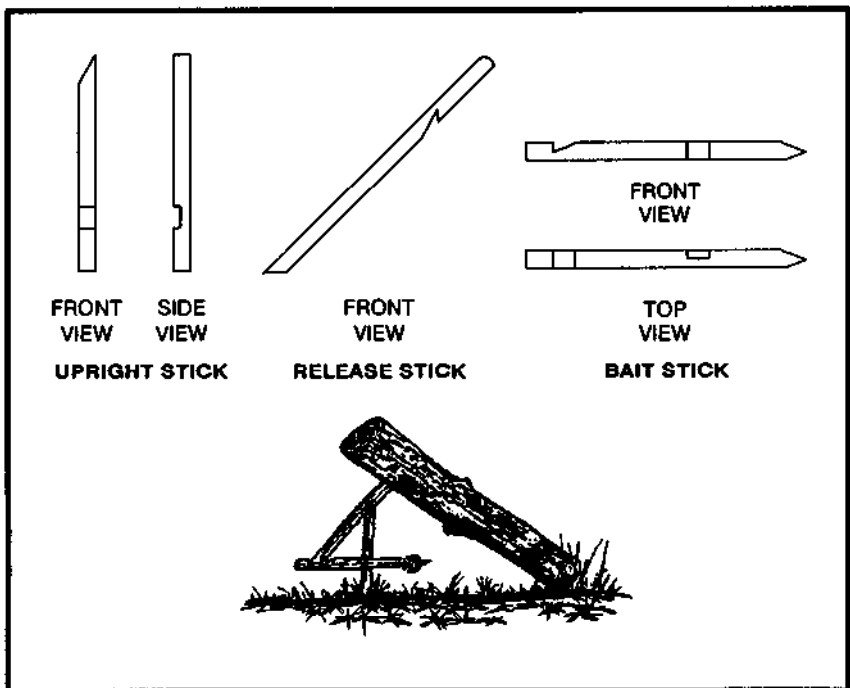
Figure 8-12. Figure 4 deadfall.
