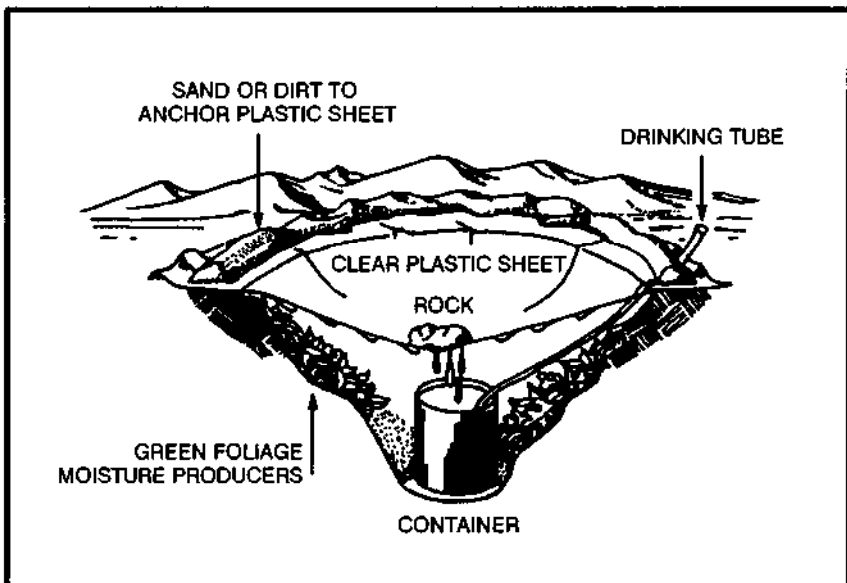
Figure 6-7. Belowground still.
