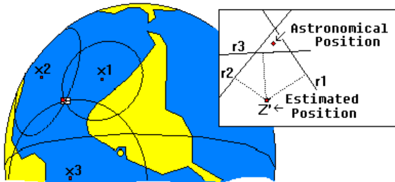
fig. 10 - Triangle formed by the intersection of three lines of Altitude
