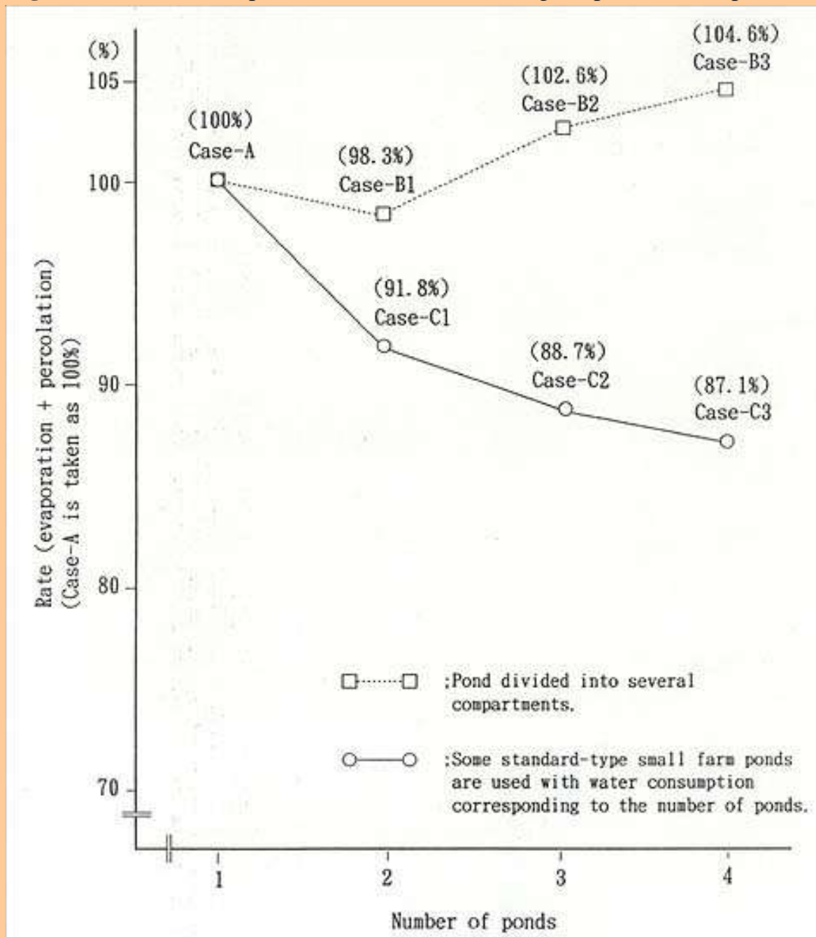
Fig.4. Effective of Compartment method in reducing evaporation and percolation
