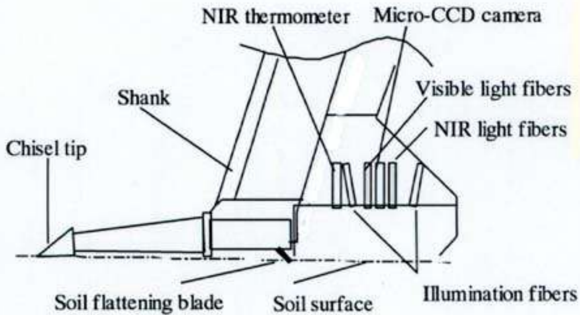
Fig.7. Soil penetrator and optical fiber probes
