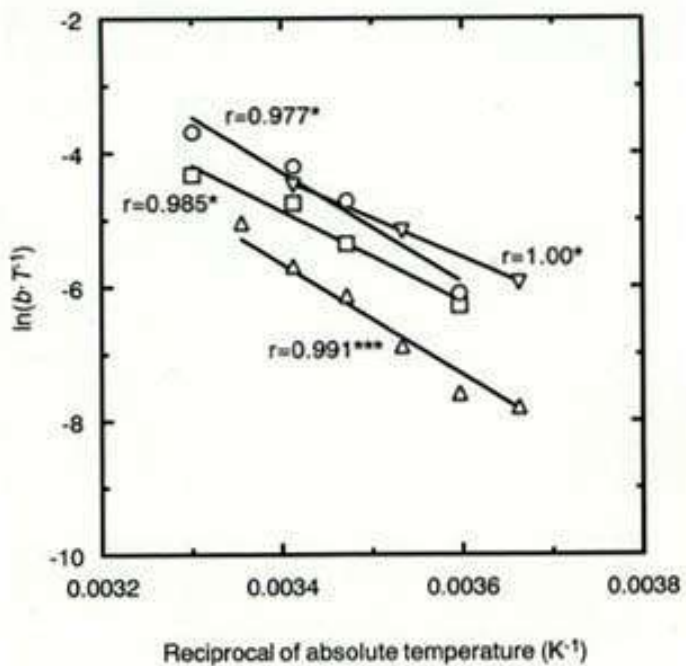
Fig. 5. Relationship between \ln(b \cdot T^{-1}) and reciprocal of absolute temperature for shredded cabbage ( \circ ), shredded lettuce ( \square ), blueberries ( \triangle ) and raspberries ( \nabla ) Solid lines denote the linear regression lines.
