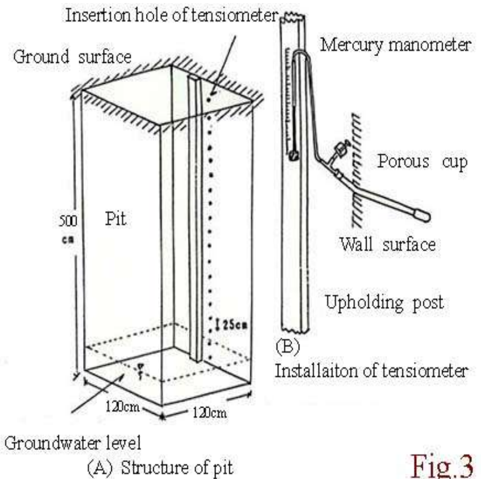
Fig.3. Method of measurement of soil moisture content 2)
