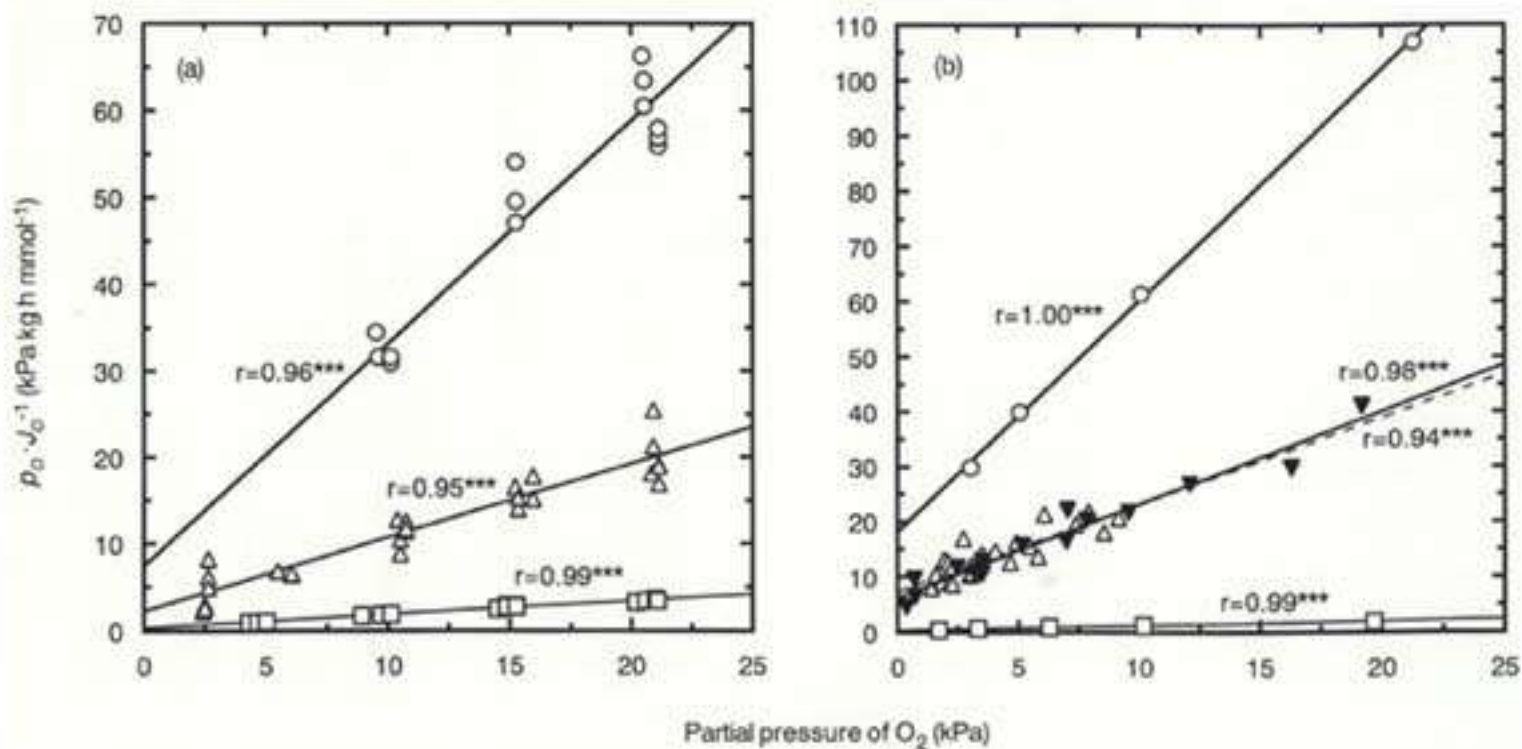
Fig. 1. Relationship between p_{O_2} \cdot J_{O_2}^{-1} and partial pressure of O_2 for shredded lettuce ( \Delta ), tomatoes ( \circ ) and broccoli ( \square ) based on the experimental data obtained in this study (a) and for apples ( \circ ), broccoli ( \square ), bananas ( \blacktriangledown ) and blueberries ( \Delta ) based on the published data (b)
