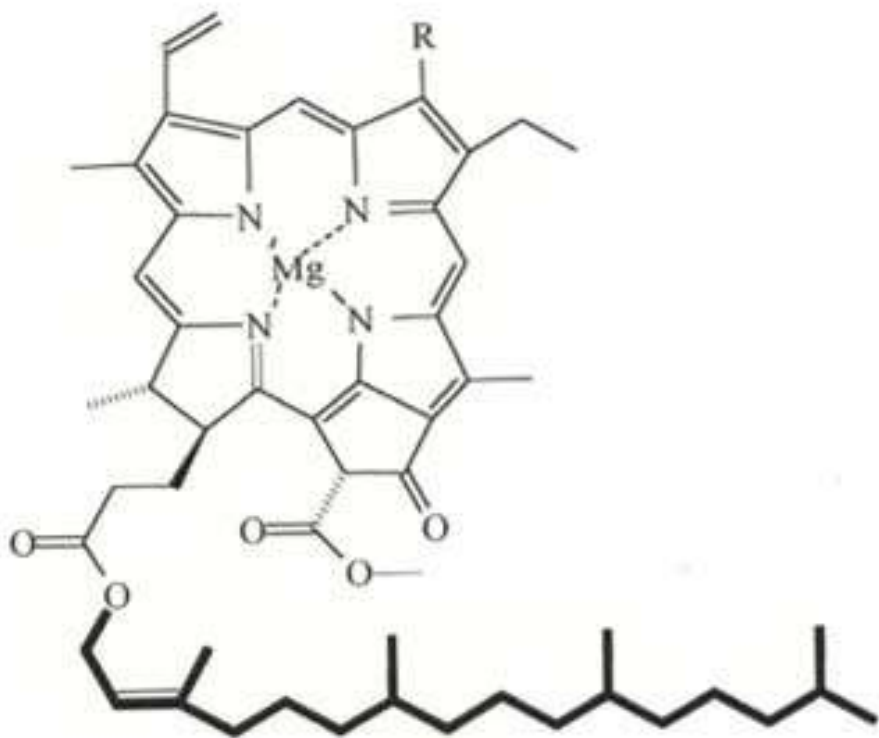
Fig.7. Chlorophyll molecule
