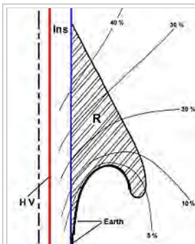
Figure 3, a rubber or elastomer body R is pushed over the insulation (blue) of the cable. The equipotential lines between HV (high voltage) and earth are evenly spread out by the shape of the earth electrode. Field concentrations are prevented in this way.
