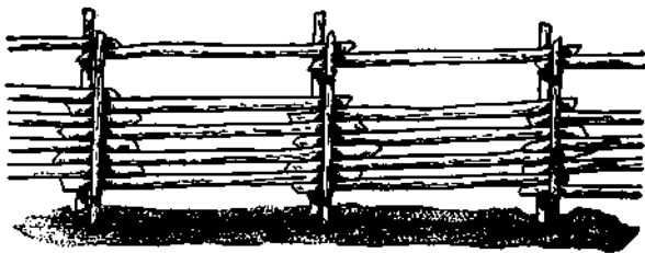
FIG. 91.—Post and rail fence.
