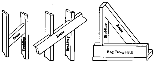
FIG. 78.—Studding braces.
