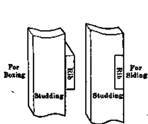
FIG. 76.—Attachment of ribs to studding.
