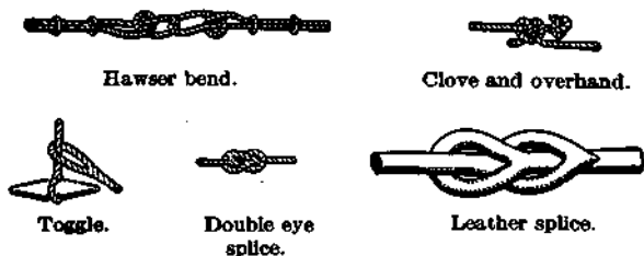
FIG. 230.—Splices.
