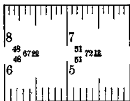
FIG. 115.—Rafter table.
