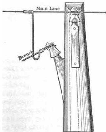
FIG. 43.—Branch-line connection. Iron wire.
