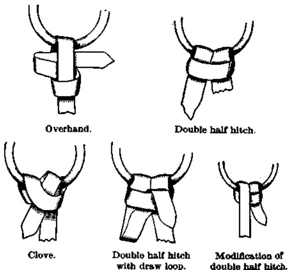
FIG. 228.—Latigo ties.
