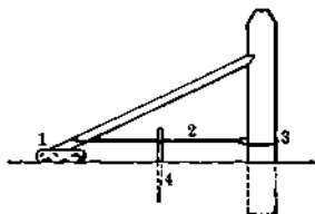
FIG. 97.—Brace for corner post.
