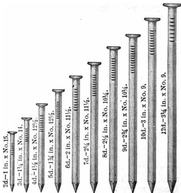
FIG. 235.—Wire nails.
