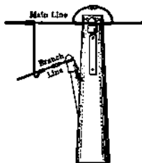
FIG. 44.—Branch-line connection. Hard-drawn copper wire.
