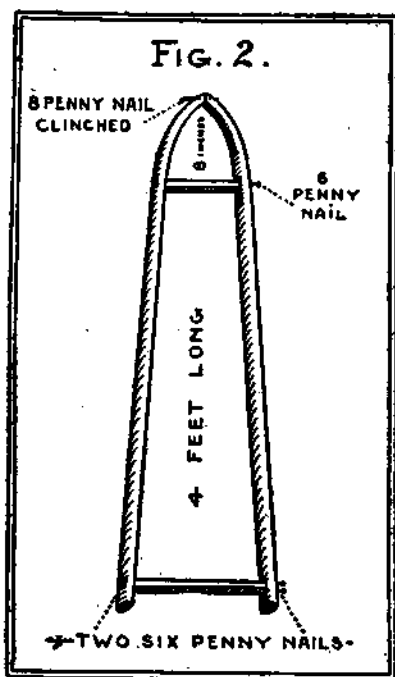
STRETCHING FRAME.
