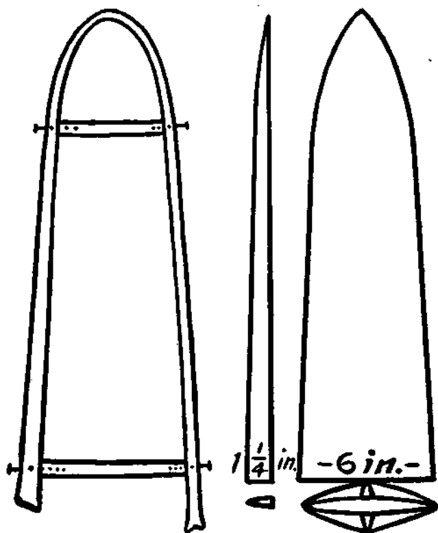
POLE STRETCHERS.
