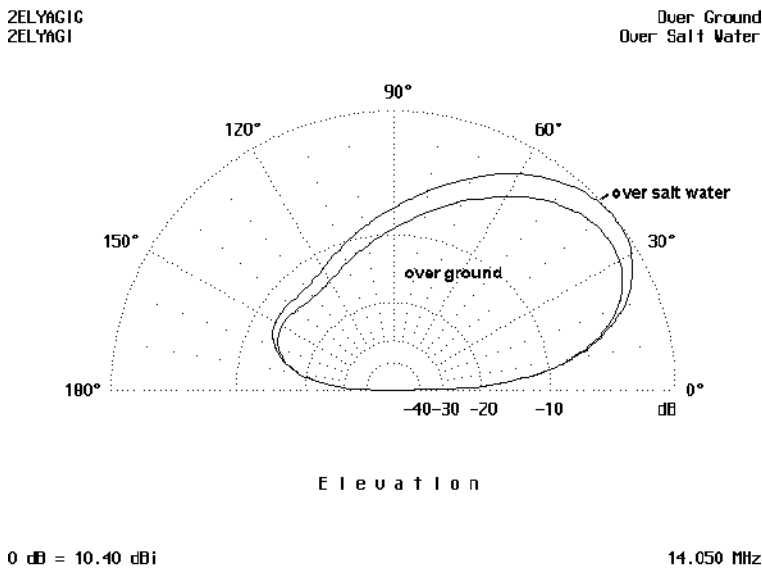
Figure 1: 2-element Yagi at 25' over land and salt water. Peak gain is 10.40 dBi (over salt water) at 38 degrees take off angle in this design.
