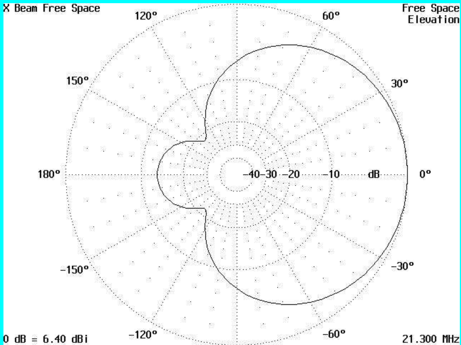
Figure 2 Elevation Pattern for X-Beam in Free Space
