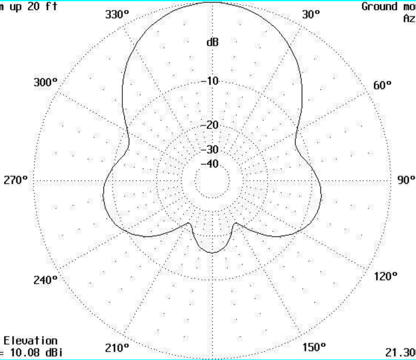
Figure 3 Azimuth Pattern of X-Beam Elevated 20 Feet Above Ground
