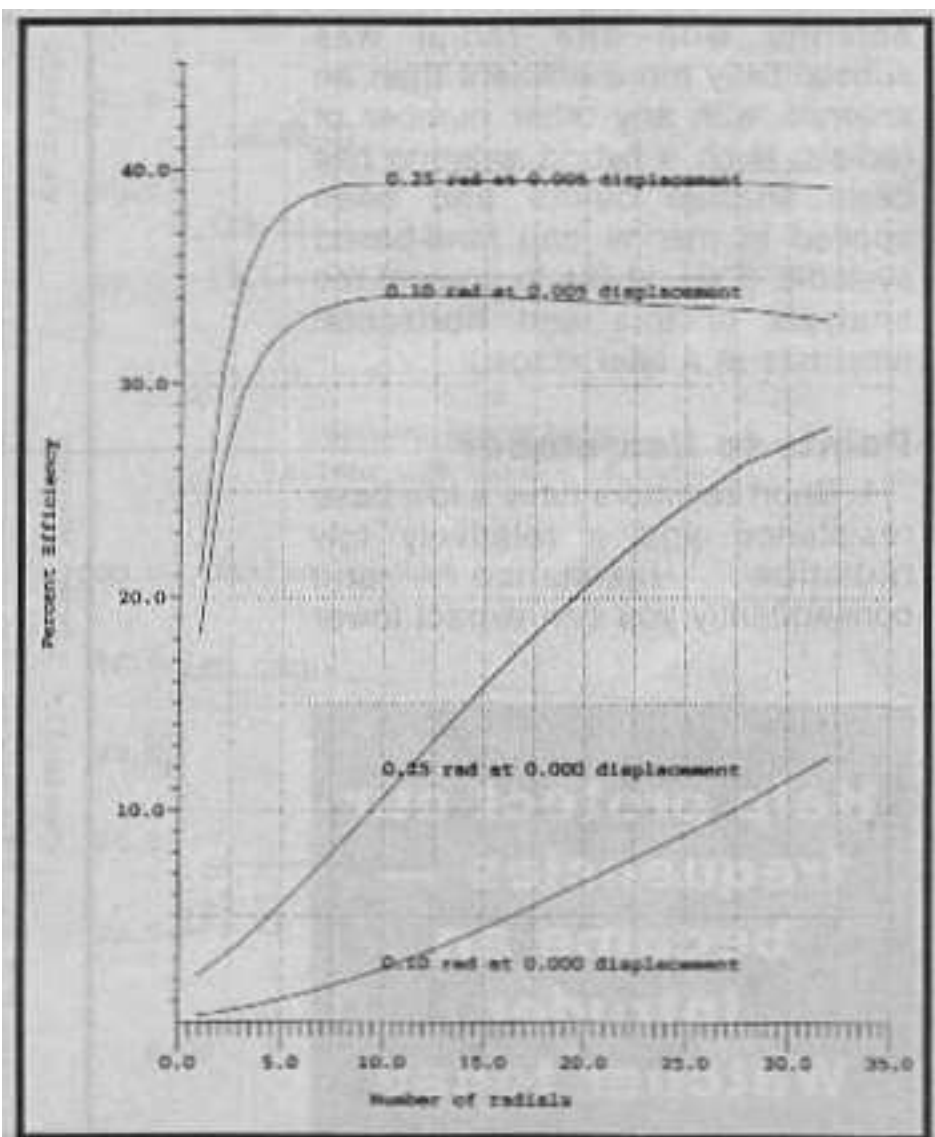
Fig 4 — Radiator/radial length and displacement.
