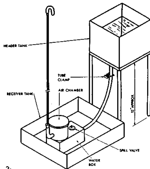
Fig. 5/8 Hydraulic ram—layout
