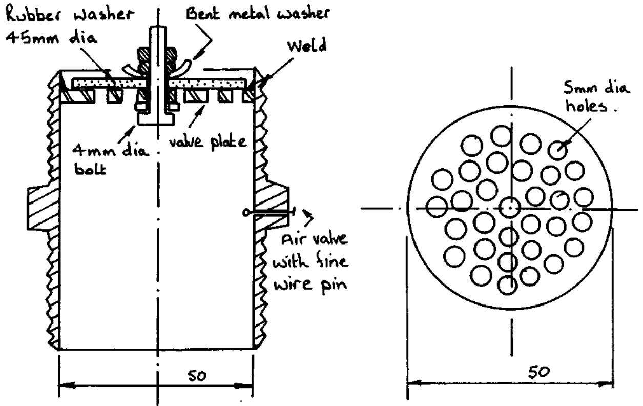
FIG.5 CONSTRUCTION OF DELIVERY VALVE.
