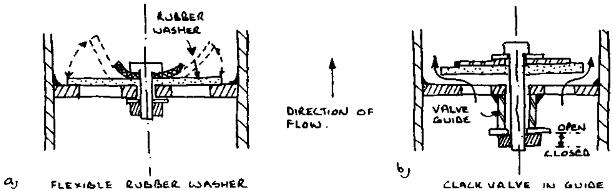
DELIVERY NON-RETURN VALVES
