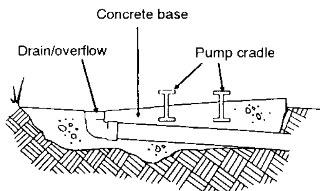
Section through pump base
