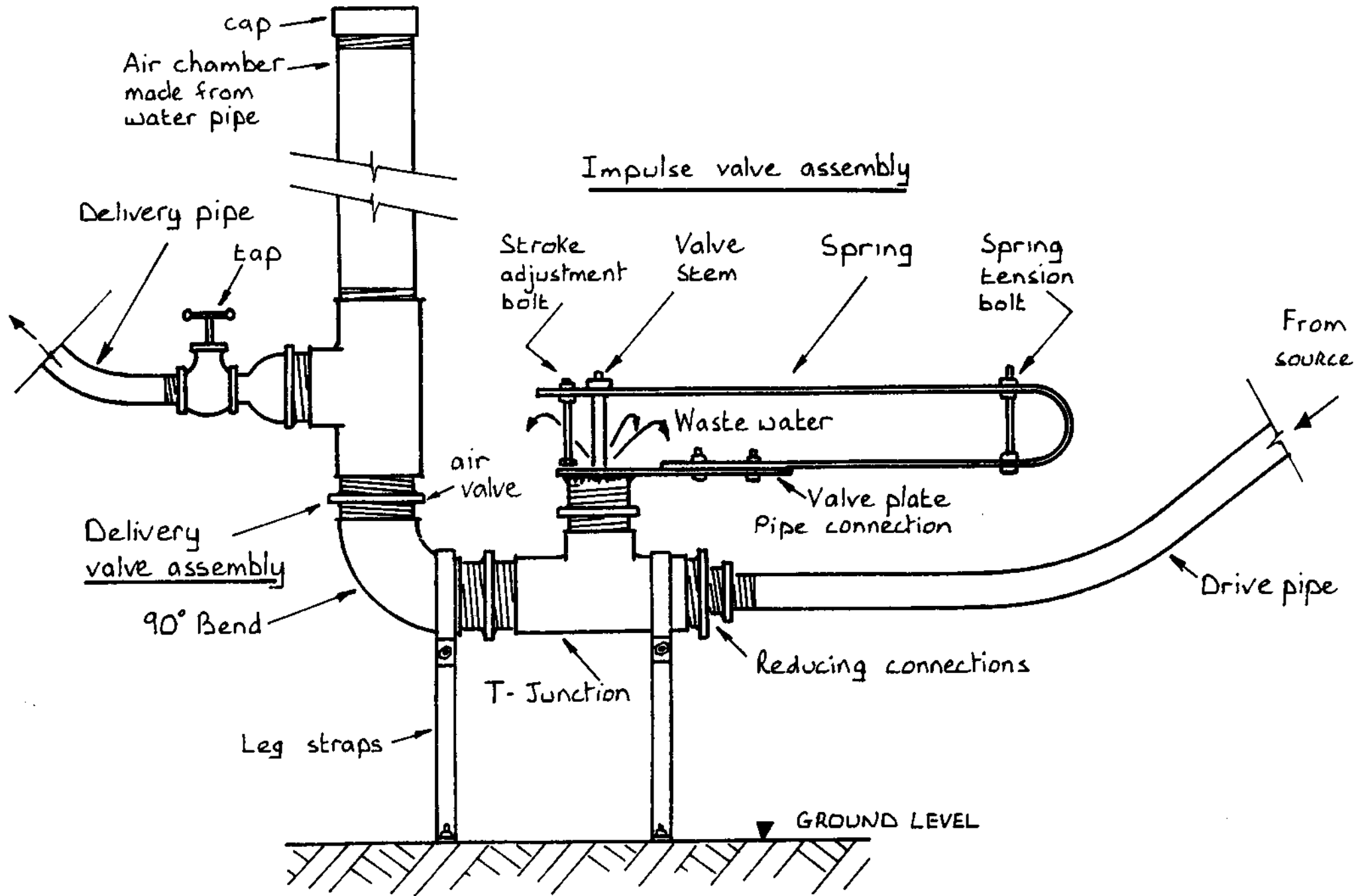
FIG 3 GENERAL ARRANGEMENT OF RAM CONSTRUCTED FROM PIPE FITTINGS
