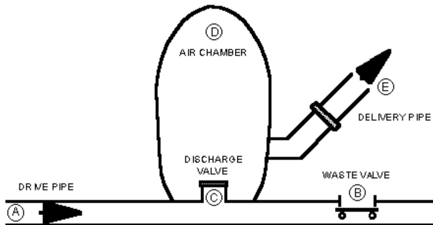
Figure 1. Hydraulic ram pump components.
