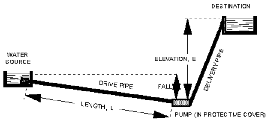
Figure 2. Hydraulic ram pump system layout
