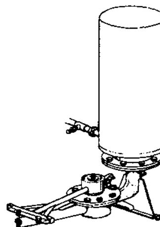
A 'DCS' RAM PUMP Nepal
