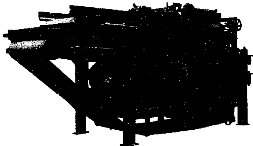
Belt filter type S7
