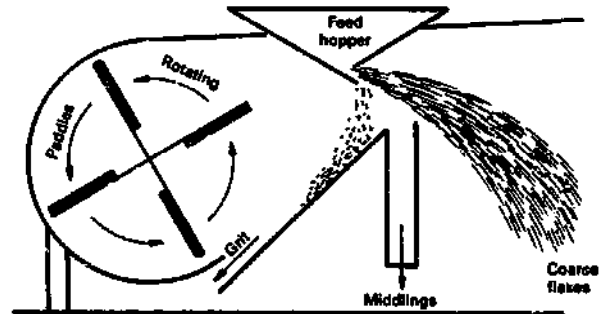
Winnowing principle
