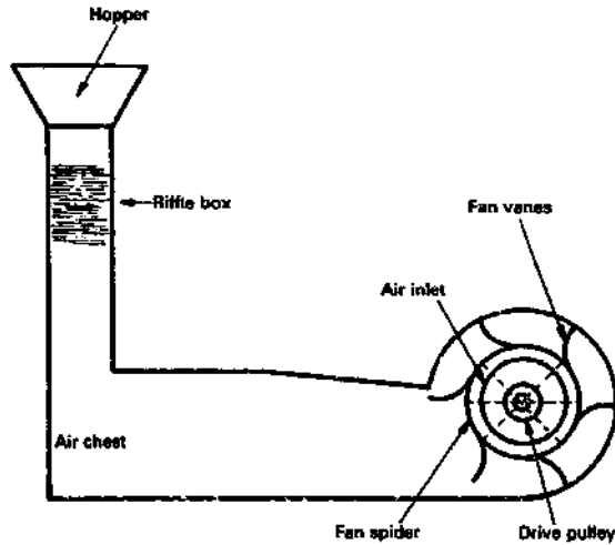
Principle of Lupa dry blower
