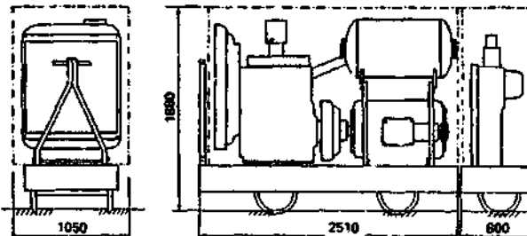
T36EP for underground use with FLP Electrical
