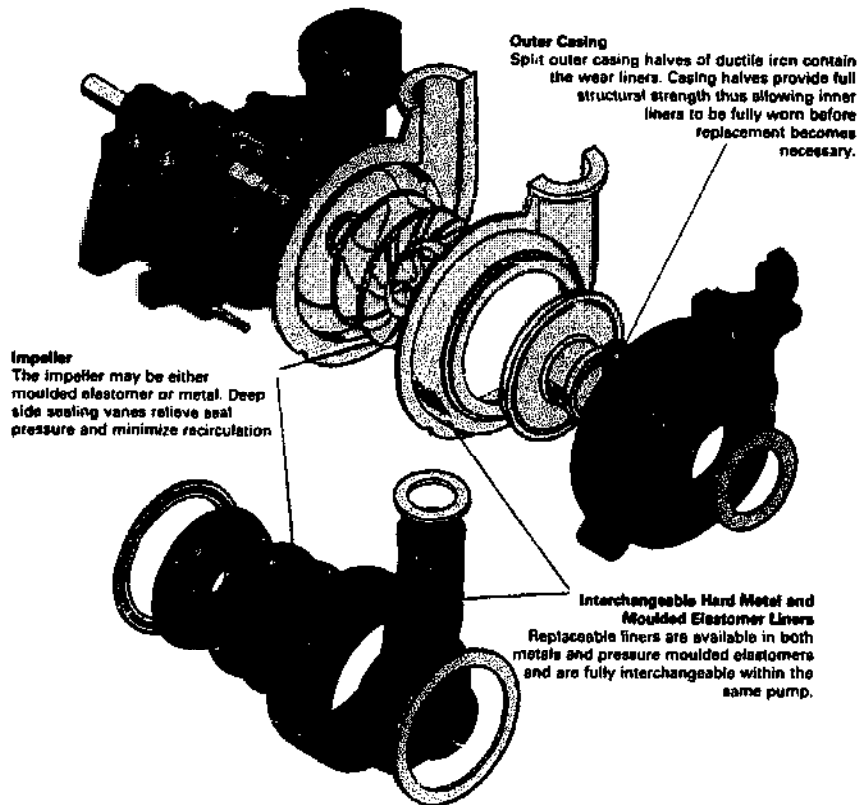
Slurry pump construction
