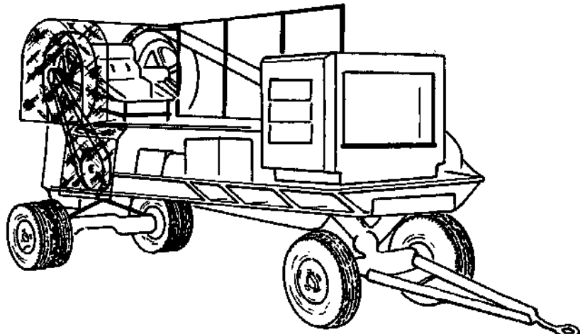
The complete mobile unit, comprising jaw crusher, rotary screen, wheeled chassis, diesel engine and drives
