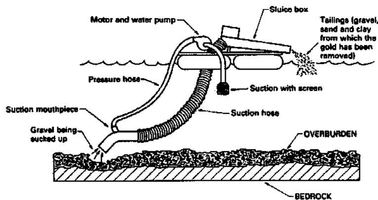
Principle of the suction dredge
