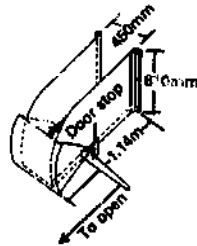
Single cut-off door for discharge end
