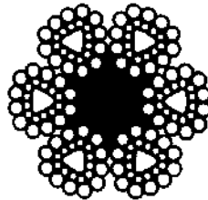
2 Triangular strand
