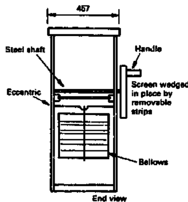
General arrangement of Mexican dry washer
