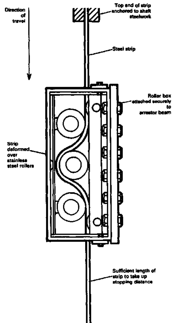
Selda principle (mine cage application)
