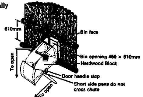
View of bin with chute fitted, using both door types in a double-door arrangement
