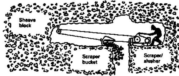
Scraper installation in underground stope
