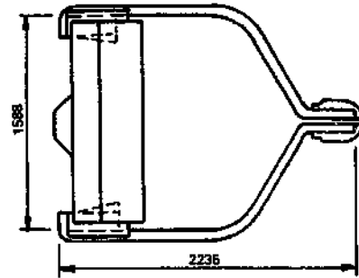
Typical scraper bucket
