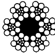
B Triangular strand
