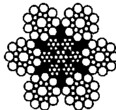
C Coal cutter and slusher ropes
