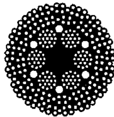
5 Superflex multi-flat stranded (non-rotating)
