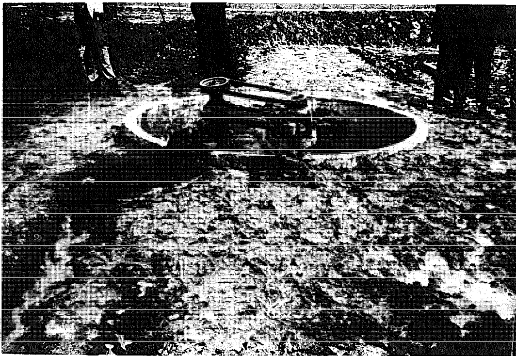
Fig. 46 Outlet of large size bio-gas plant. Effluent pumped into irrigation drain. Cheng Hsiang Production Brigade, Jiangsu Province.
