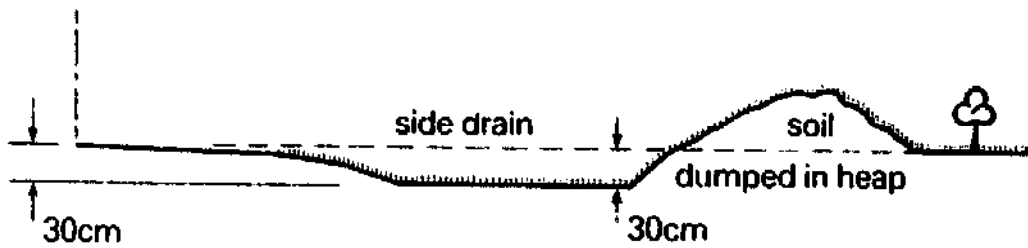
(c). Road built at ground level—incorrect.
