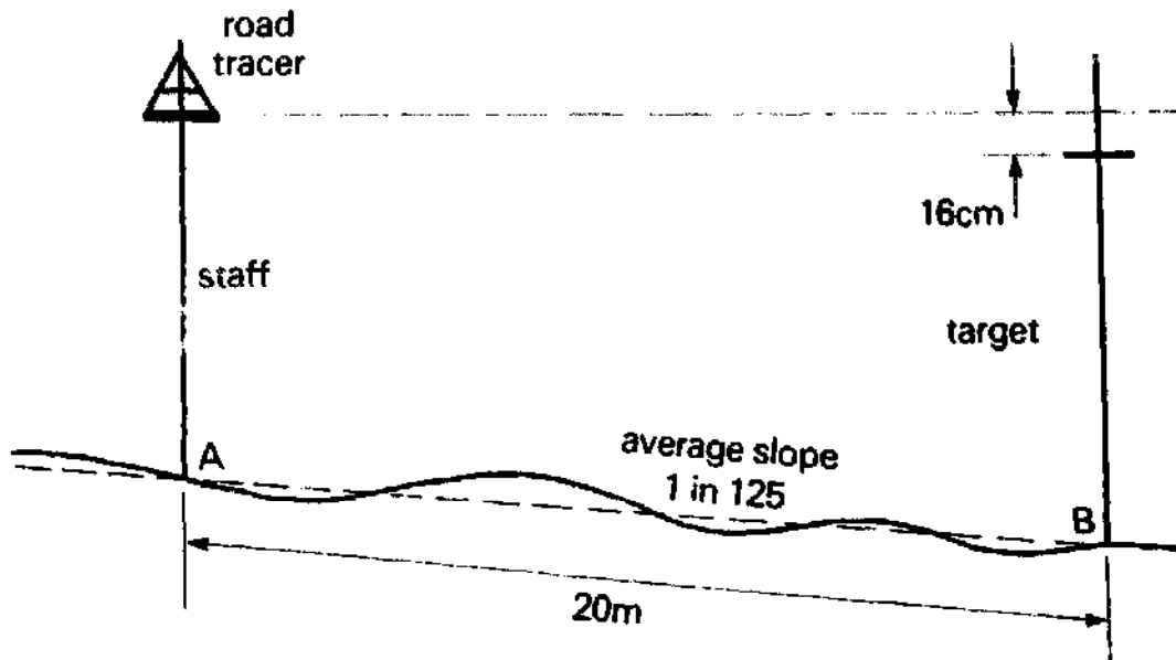
Figure A4. Use of road tracer and target.
