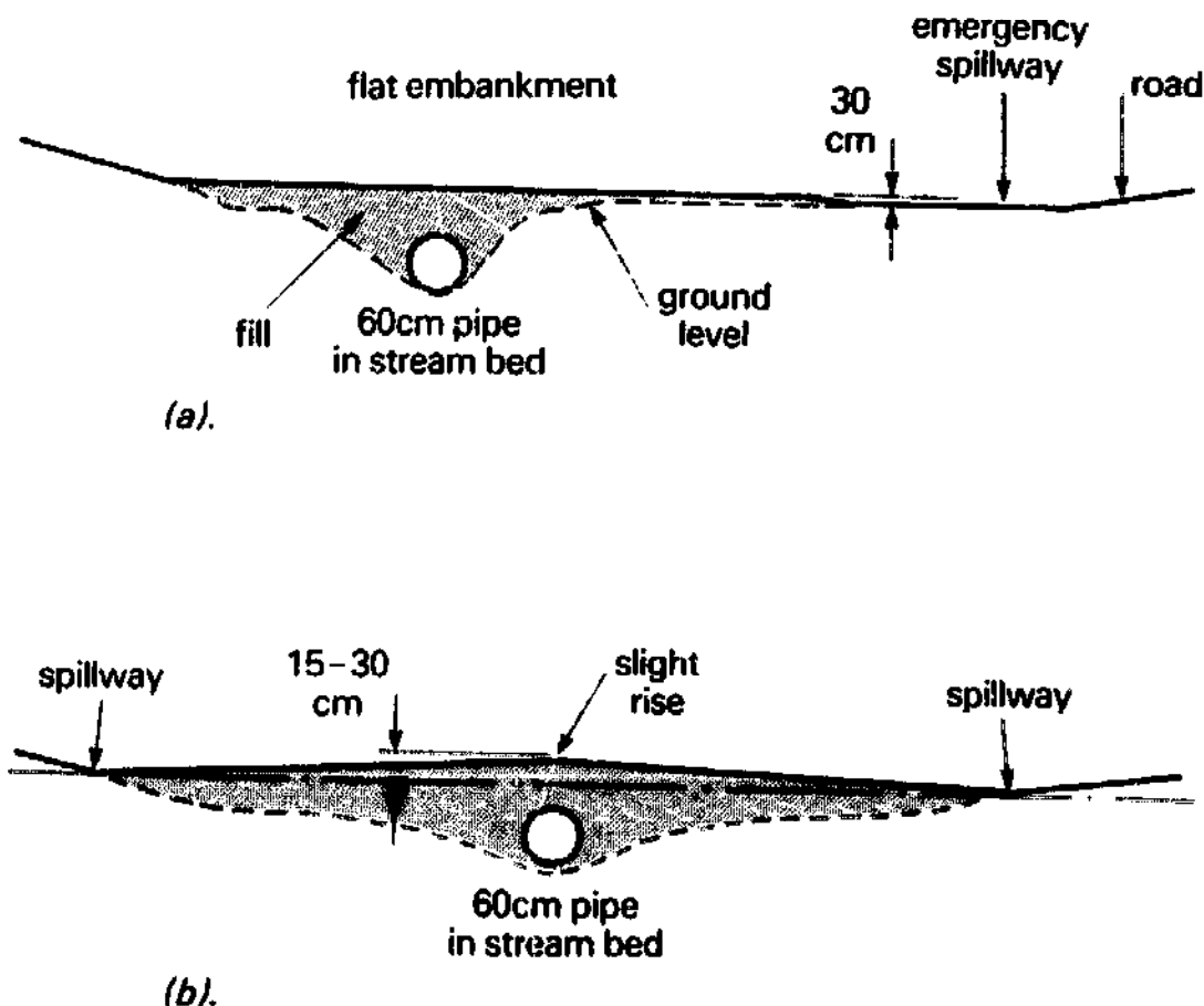
Figure 62. Use of spillway for flood protection.
