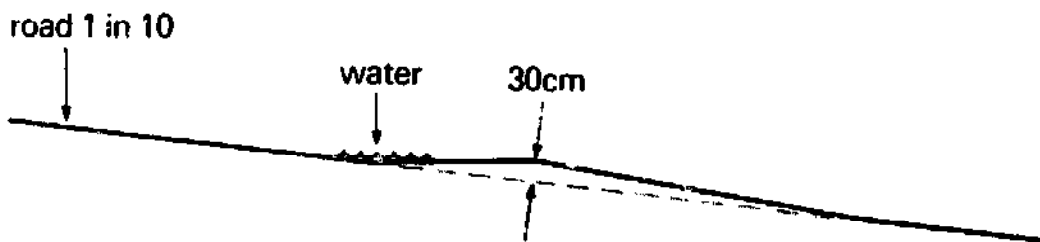
Figure 15(b). Incorrect bank on slope.
