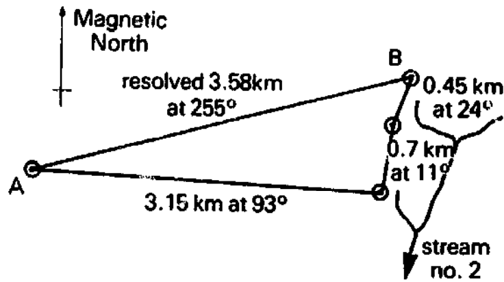
(b). Plotting the traverse.
