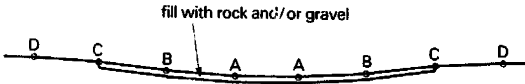
(d). Excavation for rock/gravel lining.
