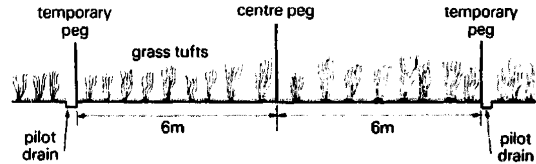
(a). Marking out.
