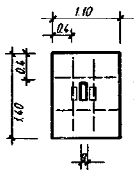
SQUATTING PLATE 1:50
