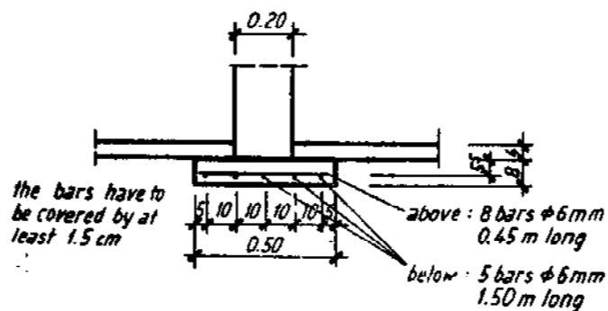
DETAIL "A" 1:20
