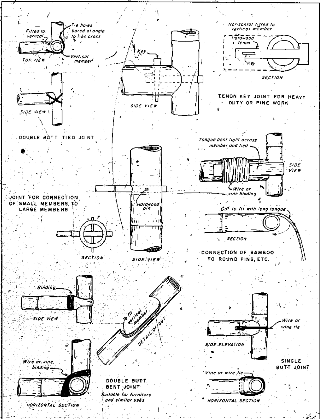
Figure 7a--Joints used in building with bamboo.
