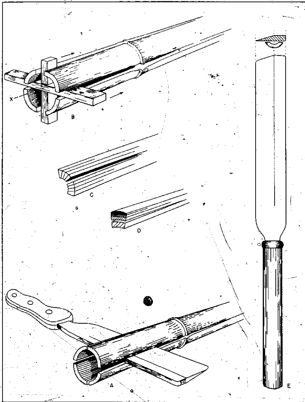
Figure 25.--Splitting of moderate-size culms to make withes for weaving and lashing. Quartering a culm; A , starting four breaches at upper end; B , driving a hardwood cross along the breaches to complete the splitting. C , dividing quarters radially, making center splits first. D , splitting radial divisions tangentially; the hard-outer (convex) strip is best, and the soft, pithy inner (concave) strip is usually discarded. E , long-handled knife used for C and D ; some workers hold a strip of bamboo on the blade to add to its effective thickness when they wish to speed up the work.
