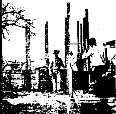
FORMS ARE HELD in alignment by vertical scaffolding tied by transverse rods. Holes left by removal of rods are plugged with dagga.
