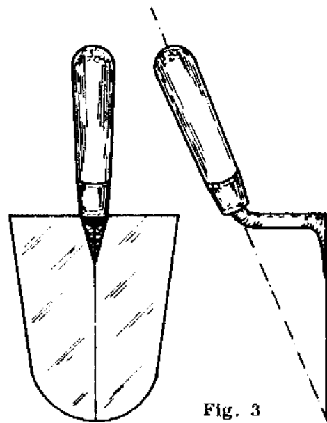
HEAVY TROWEL
