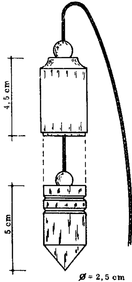
PLUMB BOB
