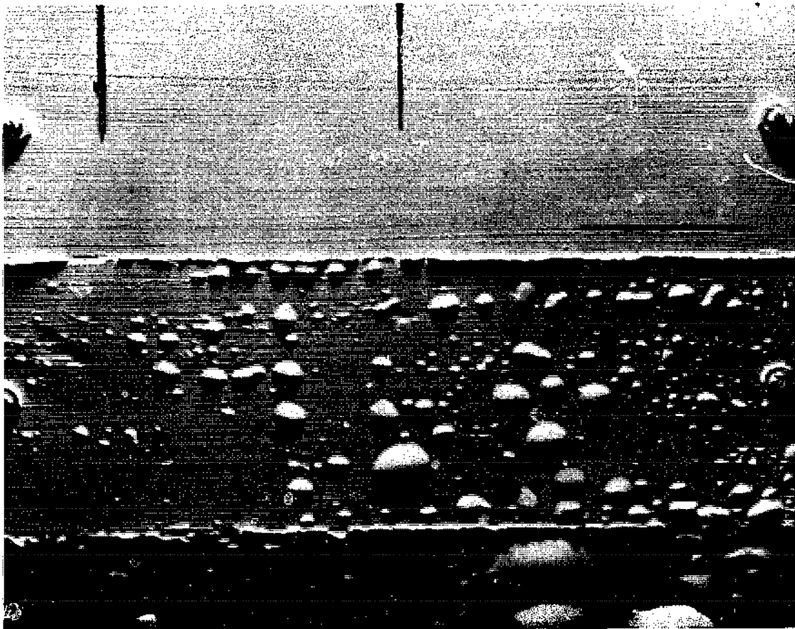
Blistering paint.
