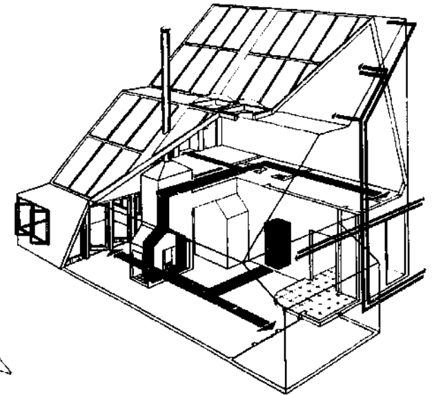
Cutaway Perspective of Solar Energy System
