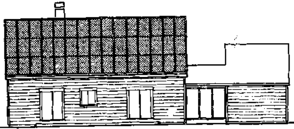
South Elevation
