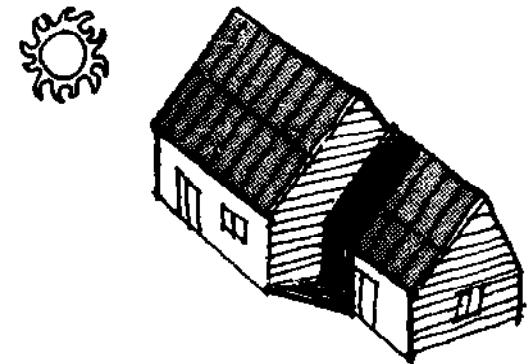
OFFSETS IN COLLECTORS CAUSE SELF-SHADING WITH RESULTANT LOSS OF EFFICIENCY AND POSSIBILITY OF COLLECTOR FREEZE-UP
