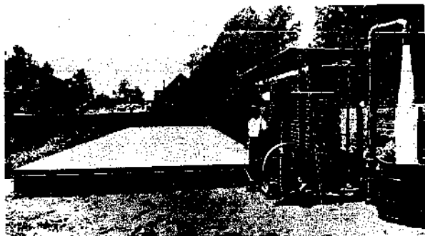
Shuman's flat-plate collector and pumping operation
