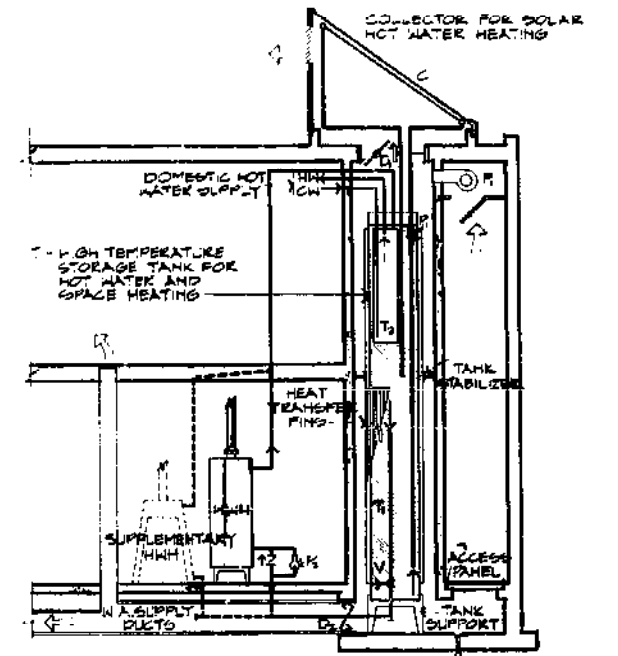
PICTORIAL SECTION ILLUSTRATING WATER HEATING STORAGE, TYPICAL PIPING, AND AIR FLOW
