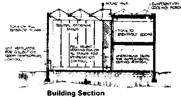
Building Section
