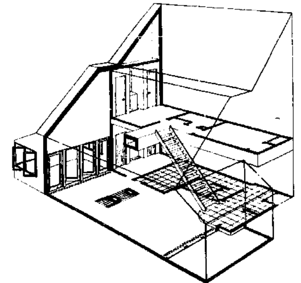
Cutaway Perspective of Living Unit
