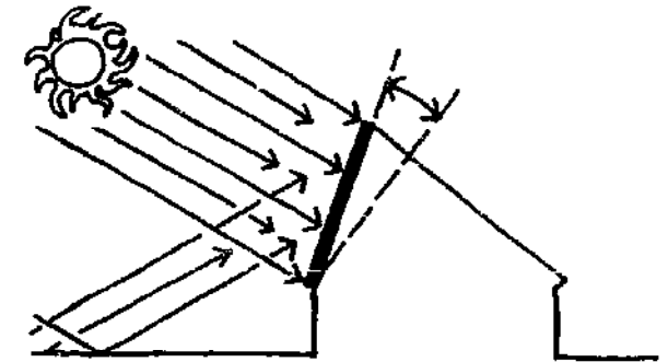
OPTIMAL HEATING ANGLE CAN BE INCREASED IF REFLECTION IS TAKEN INTO ACCOUNT
