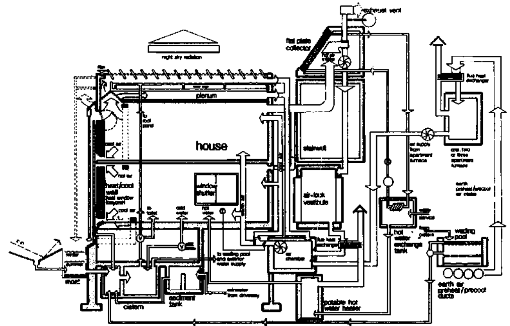
Total System Diagram for All Units
