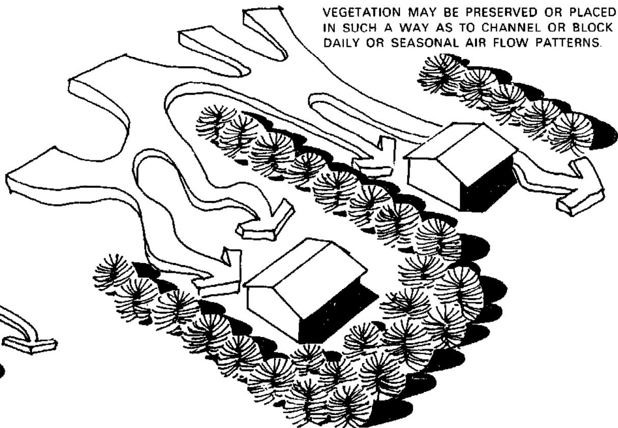
VEGETATION PROPERLY PLACED CAN DEFLECT RATHER THAN DAM COLD AIR FLOW
