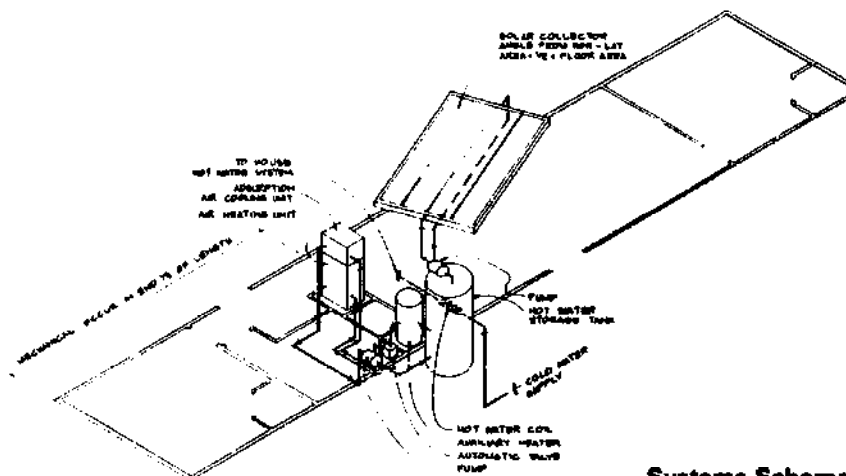
Systems Schematic
