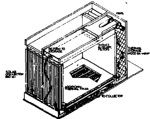
SYSTEM SCHEMATIC
