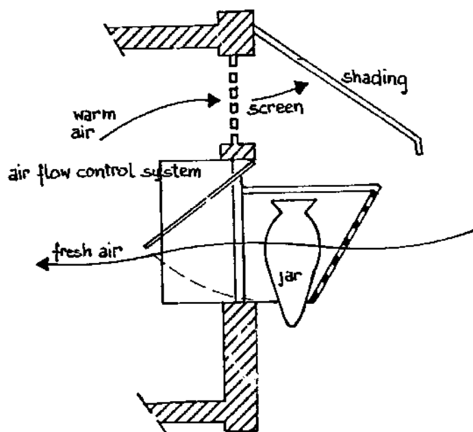
Fig. 54 An example, how the humidification can be realized in combination with a window
