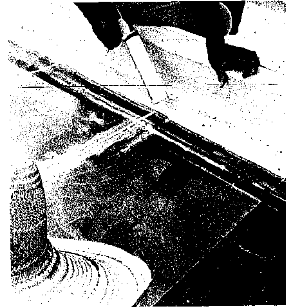
Fig 8: Glass installation. Glass panes were positioned between adjacent curb walls with 1/16 to 3/32 inch gaps between panes. Silicone sealant was then applied in a single bead along each end and in the gap separating the panes.
