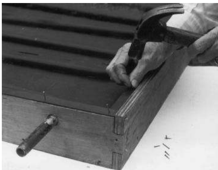
Fasten rubber strips over the rebates of sides A-B-C and D.
