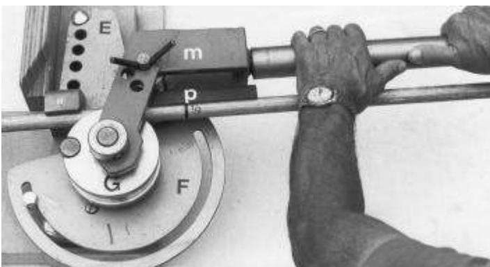
Pipe and lever are now in parallel position.
