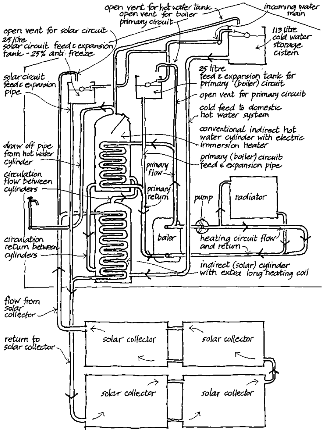
Plumbing diagram for solar collector
