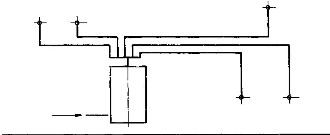
Single tap system (effective system; hot water is fastly available)
