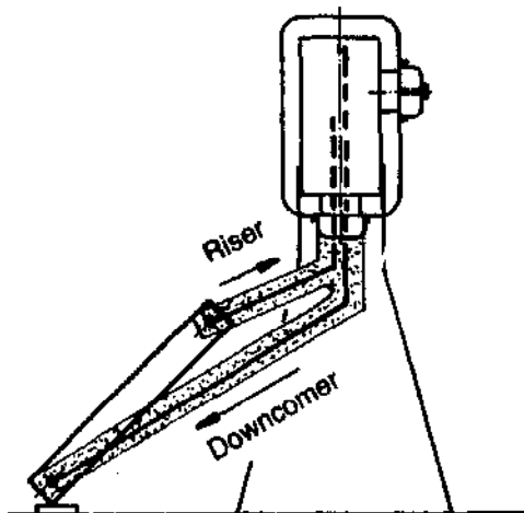
Circulation pipes of solar water heaters
