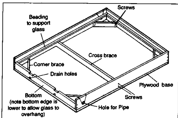
Fig. 3: The basic design for the box - which can be adapted to house either design of collector you make.
