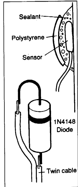
Fig. 17: Sensor construction and mounting
