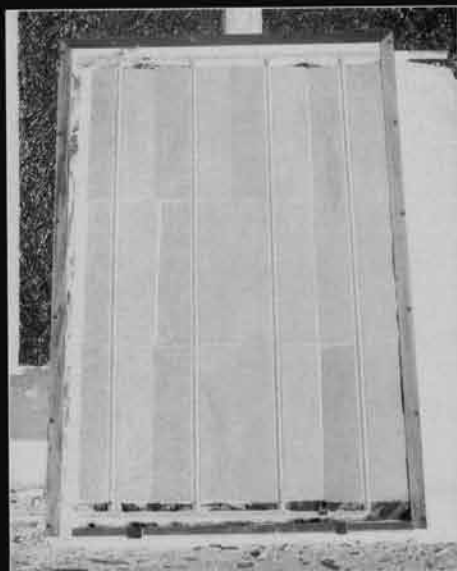
Fig. 4: The completed clip fin model solar collector, shown being made on the following pages.
