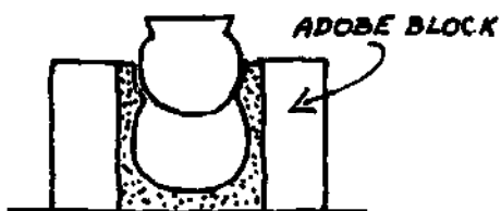
CROSS-SECTION, FIREBOX
