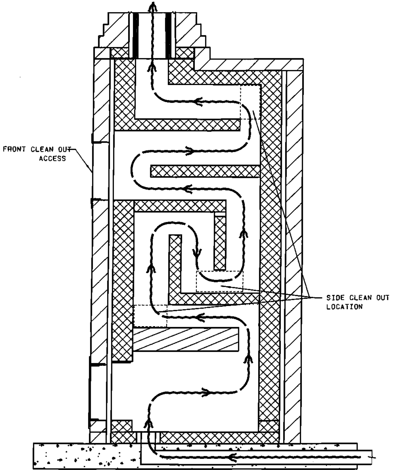
MASONRY STOVE WITHOUT OVEN VERTICAL FLUE RUN
