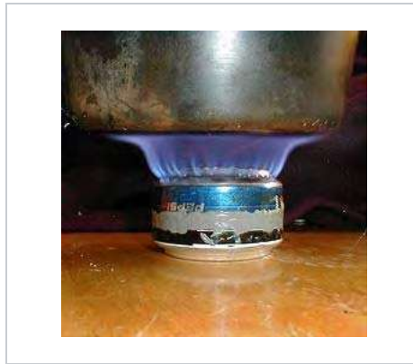
A beverage-can stove; the pot stand is omitted for clarity
