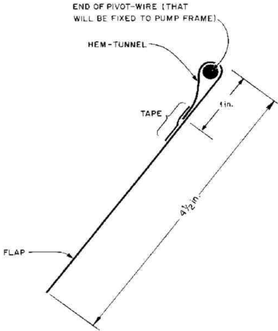
Fig. 7. End view.
