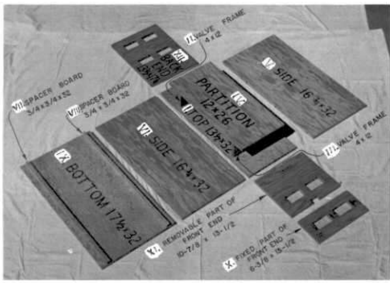
Fig. 12. Parts of the Pump "Box", with Dimensions in Inches. The Roman numbers give the best tested order for attaching these parts to each other.
