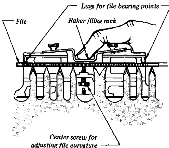
Jointing the cutter teeth.
